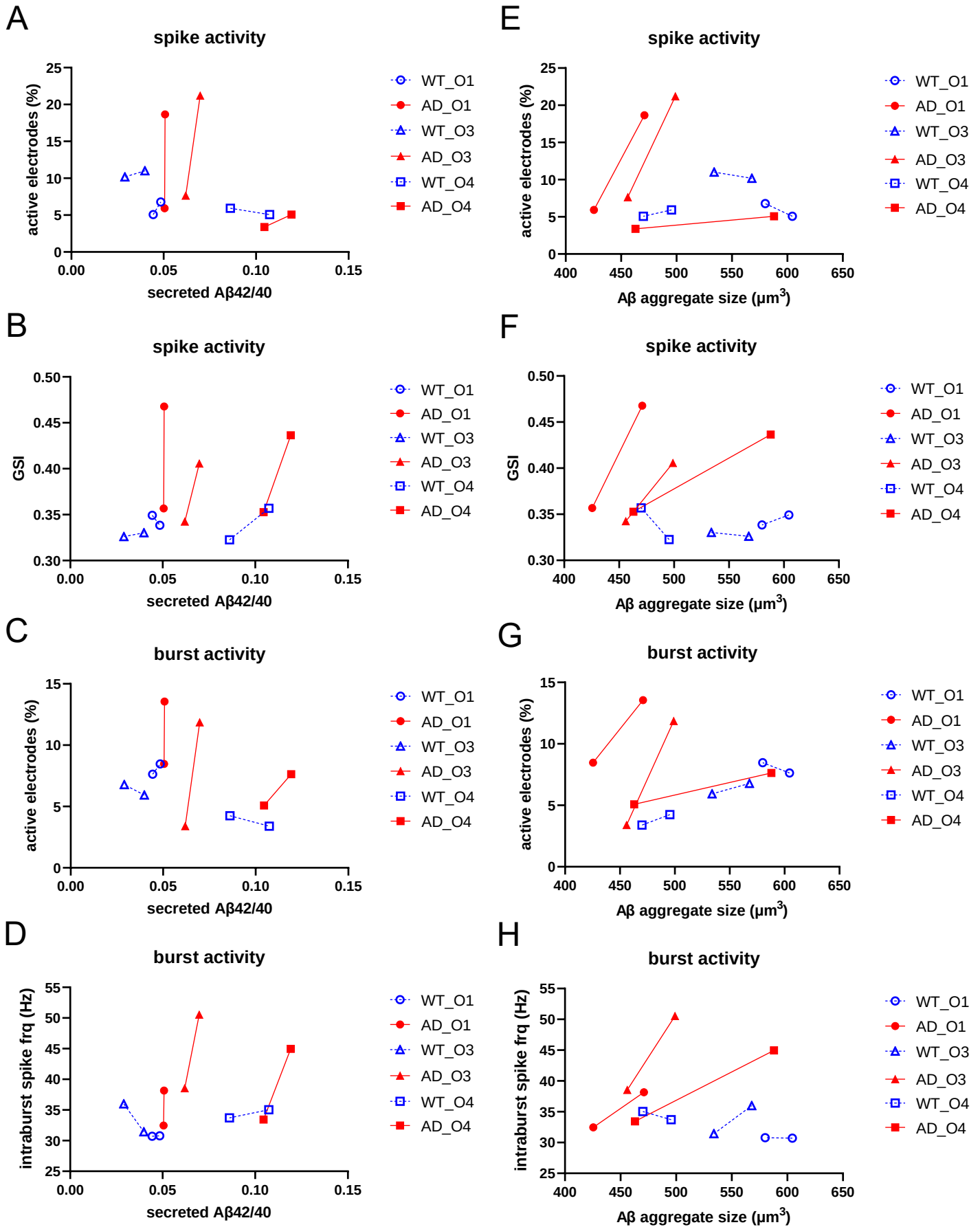
Supplementary Figure S1: Correlation between the electrical activity and A \beta in WT and AD cerebral organoids from three independent differentiations - data in absolute values.
