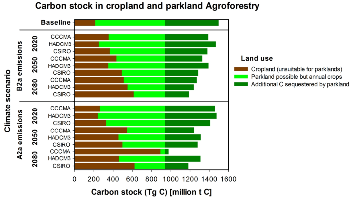
Supplementary Figure SF3. Carbon stocks in Sahelian agricultural land, assuming that mature parklands exist on the maximum possible area, for the baseline and 18 future climate scenarios. In all scenarios, the total cropping area is assumed to remain unchanged. The length of the brown bars indicates carbon stored in areas that are unsuitable for parkland, the brown + light green bars are the carbon stock in treeless cropland, and the dark green bars are the amounts of additional carbon that could be stored in parkland compared to treeless cropland.
