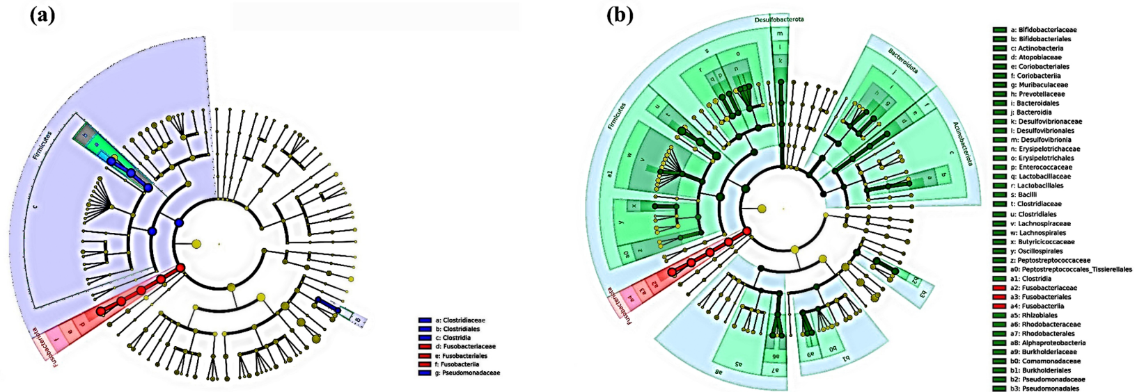
Supplementary Fig. S2 LefSe analysis of intestinal flora in hybrid sturgeon after microplastic ingestion. a-b LefSe cluster diagram of different hybrid sturgeon groups after microplastics ingestion
