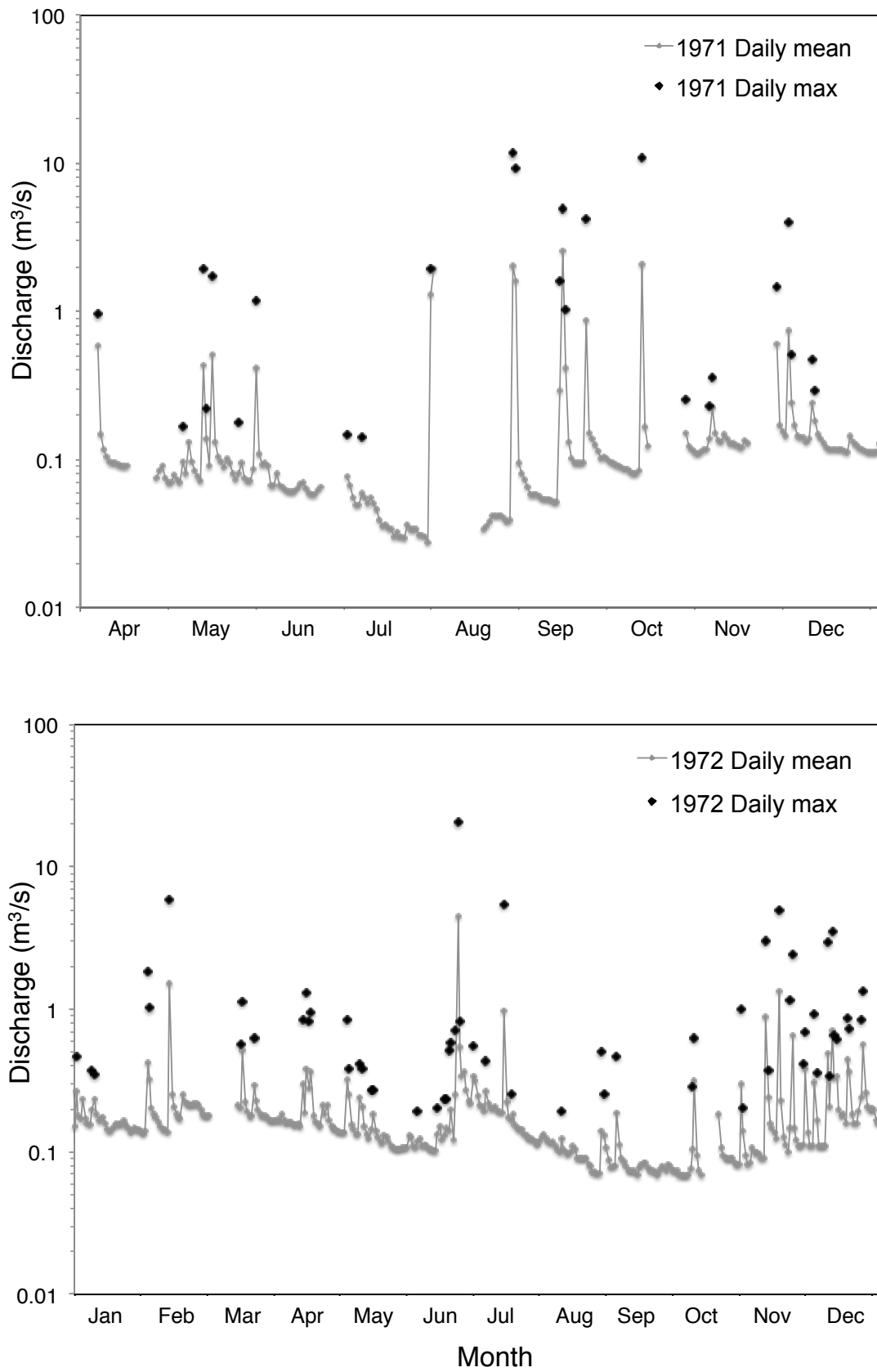
Suppl. Fig. 2 Daily mean streamflow for White Clay Creek during 1971 and 1972 and maximum flow (black diamonds) when \geq 1.5 times baseflow. There was no significant precipitation in data gaps
