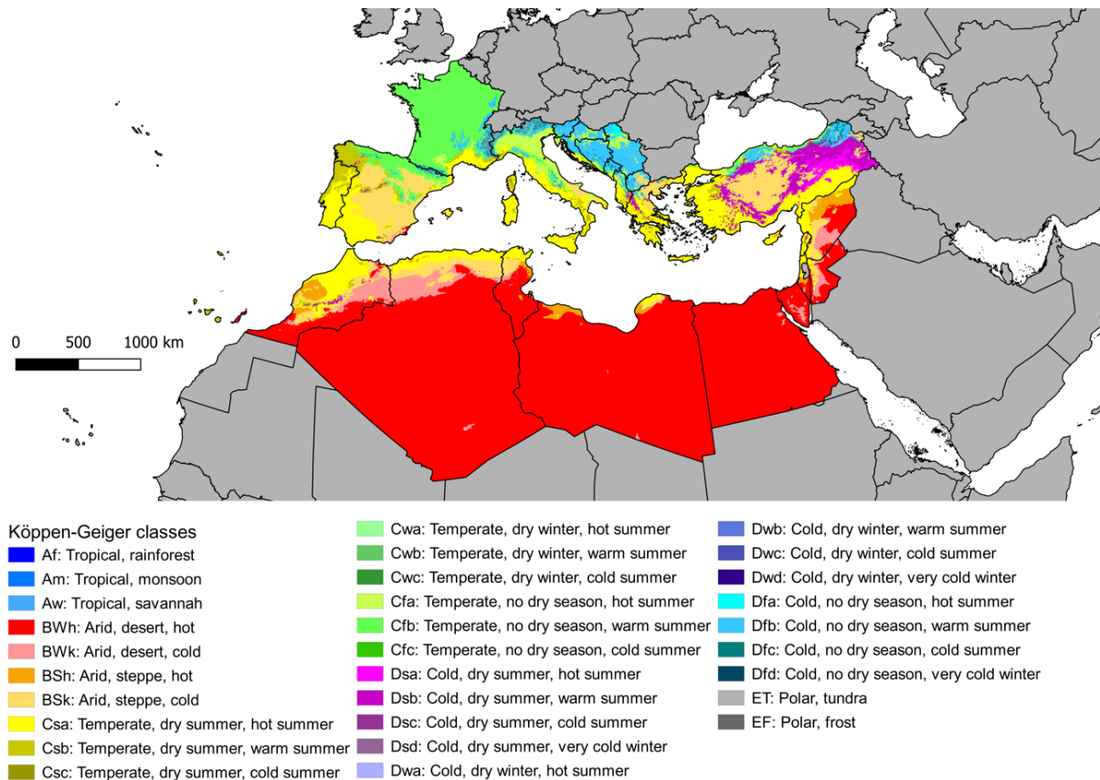
Online Resource 3. Köppen-Geiger climate classification system in the circum-Mediterranean region.
