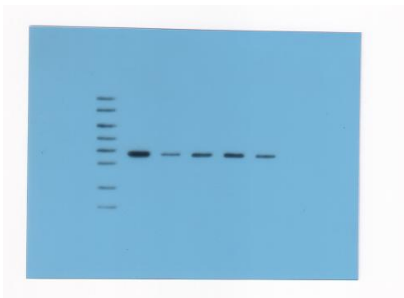
Fig 6C-2 \beta -actin
