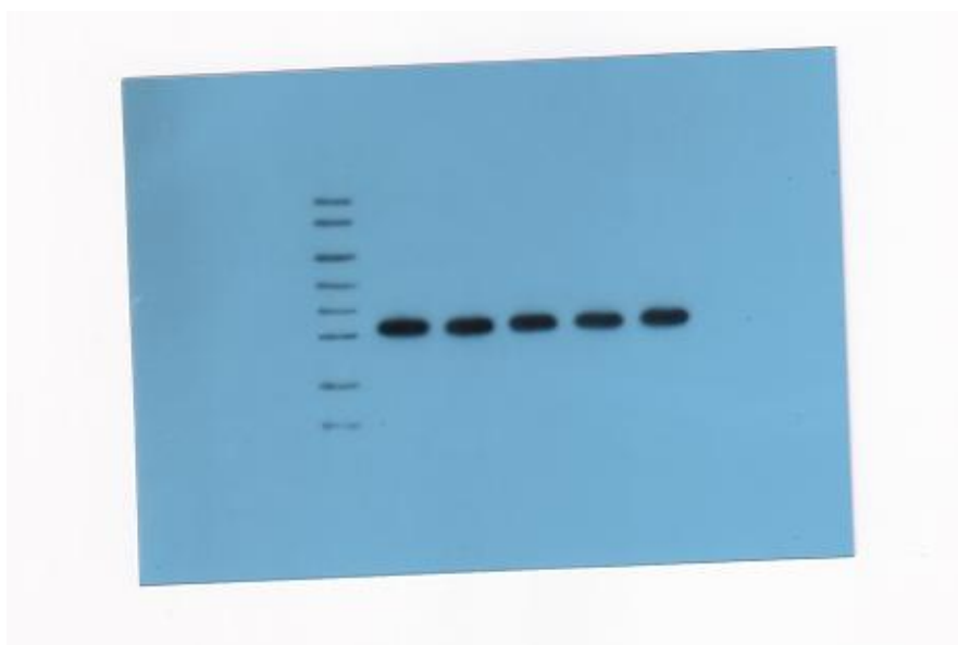
Fig 6C-2 \beta -actin
