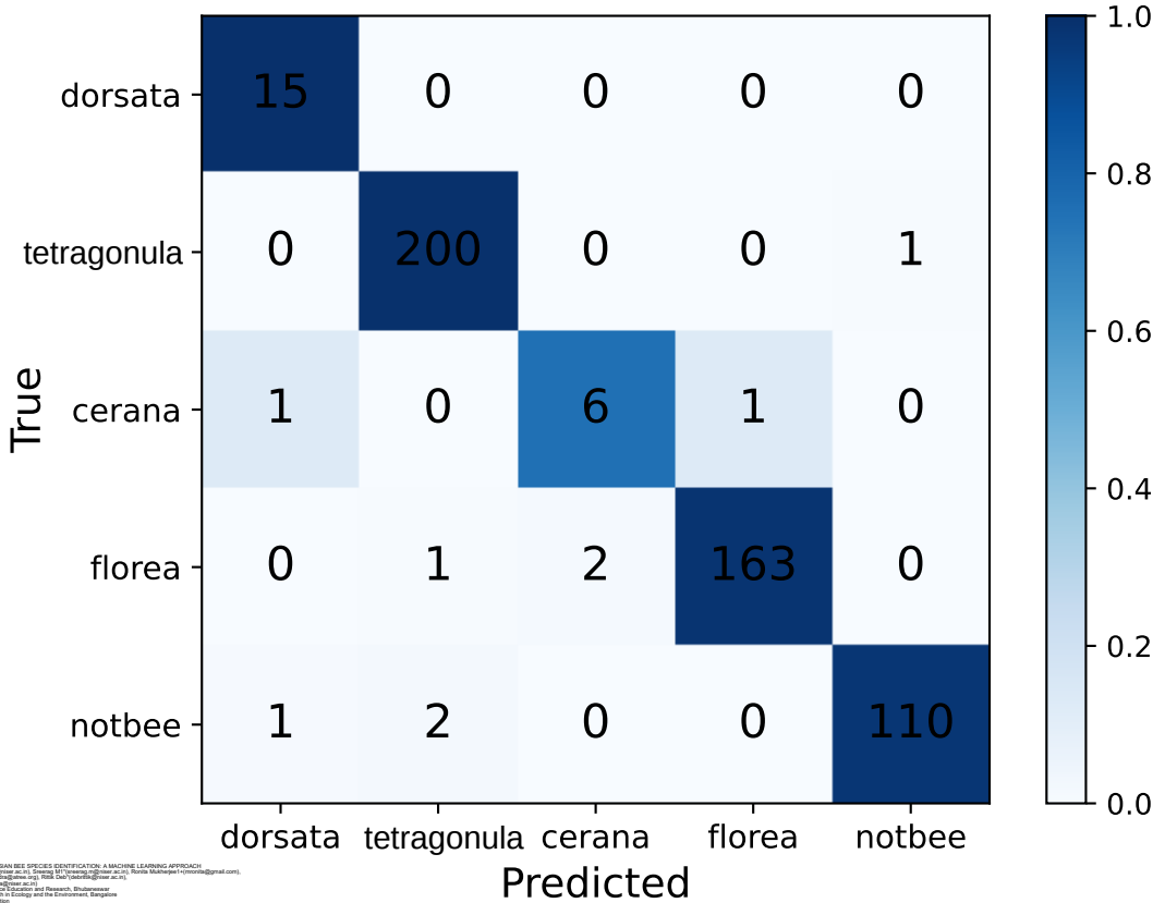
woboc: ResNet50
