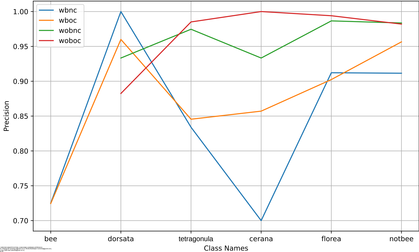
Precision for Model: MobileNet -V2
