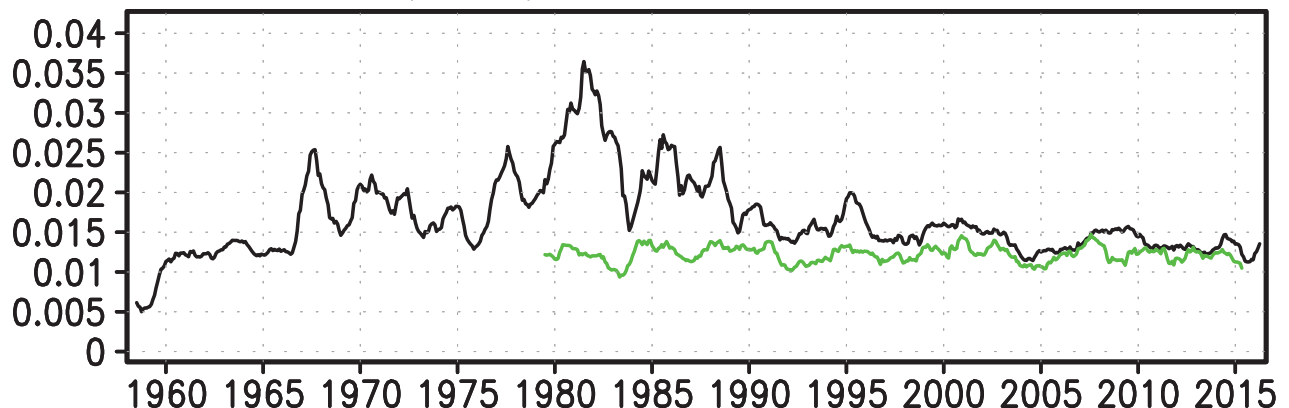
Total precipitation on divided basin
