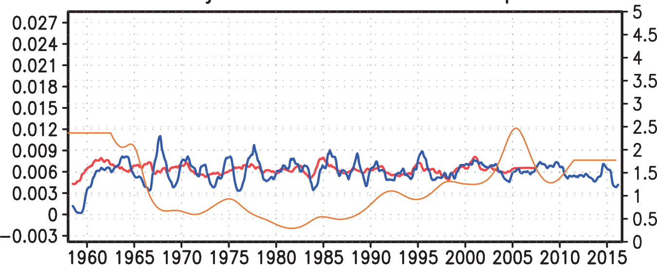
Total precipitation on divided basin
