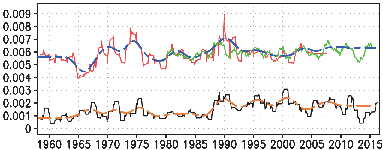
Time series of river discharge & adjustment factor for runoff input
