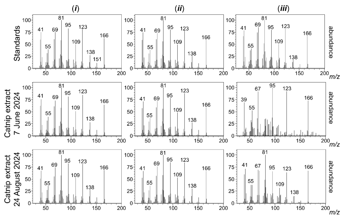
Fig. S1 Mass spectra of standards of nepetalactone isomers (iridoids i-iii ) and matching peaks detected at the same retention time in catnip extracts, related to Fig. 3c.
