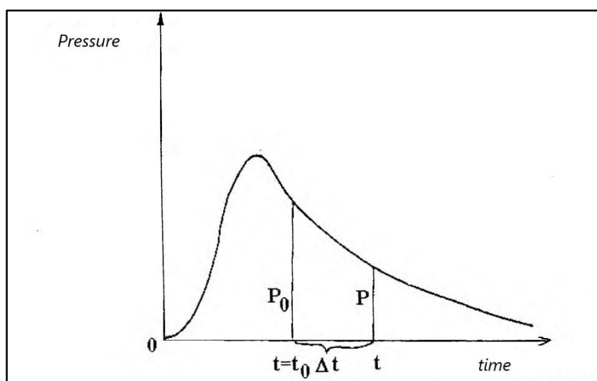
Figure S1 -Typical view of the vacuum degassing curve under continuous pumping conditions.
