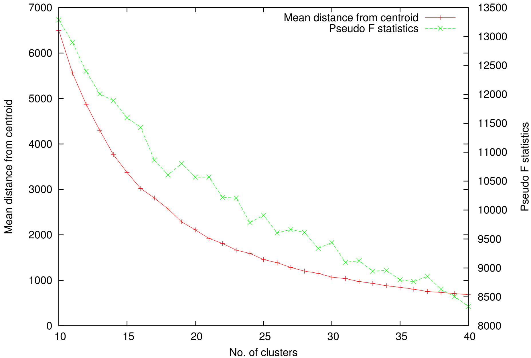
Cluster quality metrics
