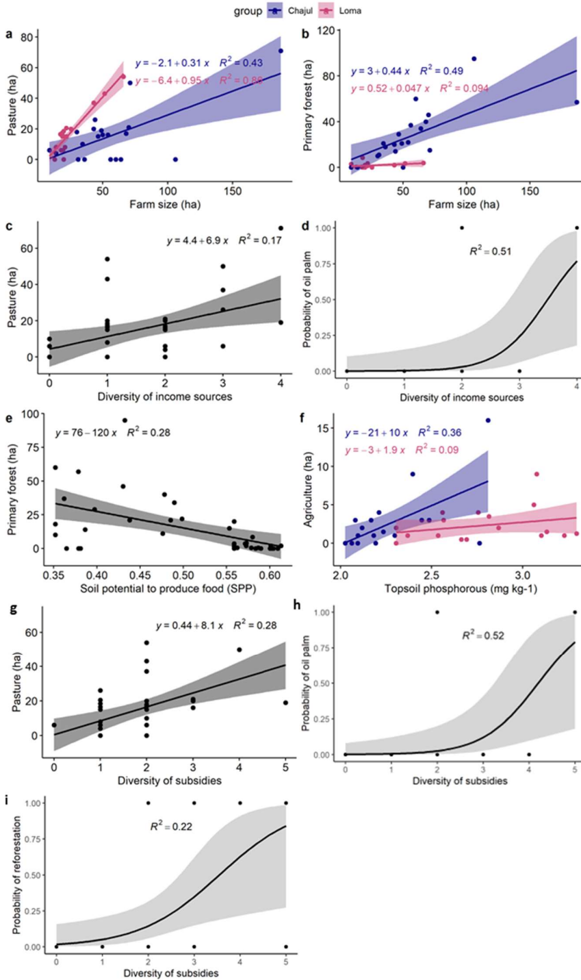
Fig. 1 Generalized linear models showing the social-ecological drivers that had a significant effect on smallholders' land-use decisions in Chajul and Loma at the local-household level (a-d), regional-biophysical level (e-f), and national-institutional level (g-i). Purple represents Chajul,
