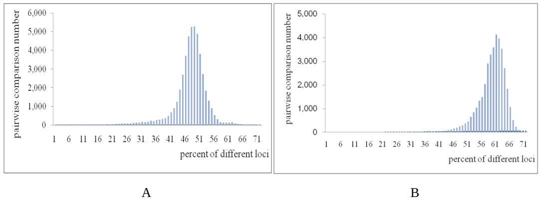
Figure S1 Distribution of different locus percentages obtained by pairwise comparisons of A 309 inbreds and B 276 hybrids
