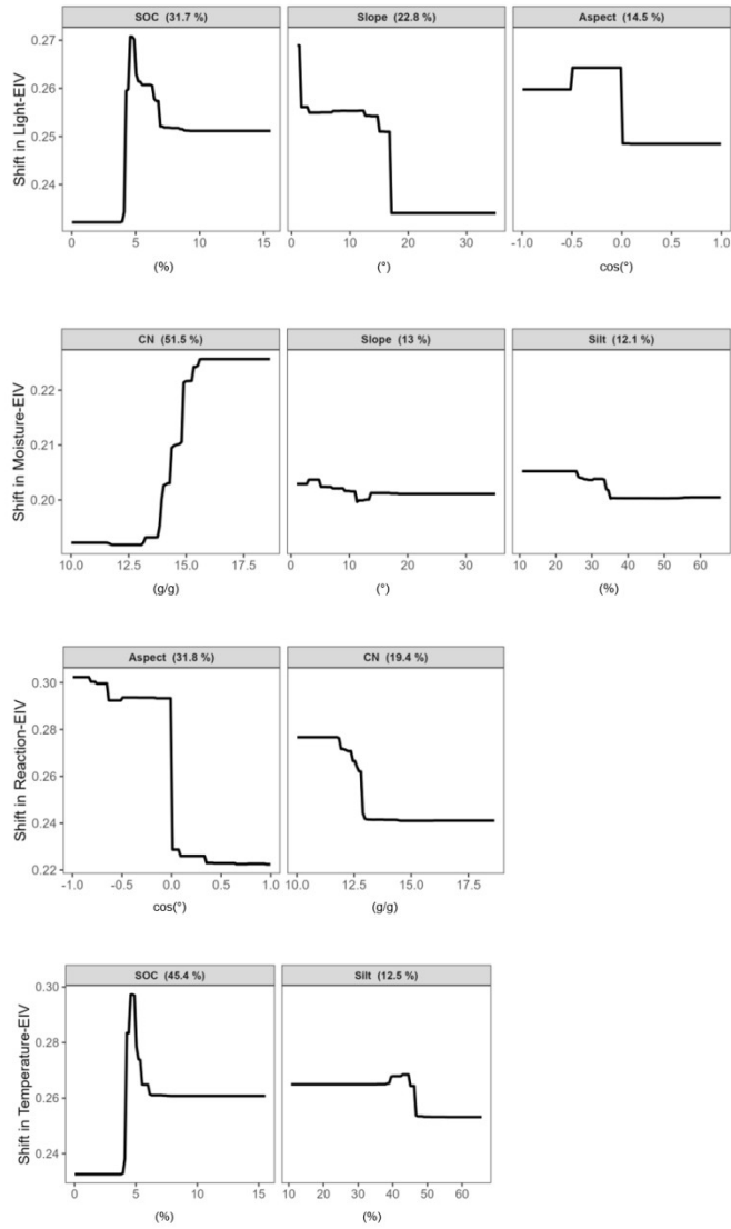
Fig. S2: Partial dependence of the most influential predictors (relative influence >10%), showing marginal effects (averaged over all other predictors) on functional-type change metrics between the two surveys: (a) strategy types, (b) life form, (c) longevity, (d) leaf traits, (e) Indicator Values. Predictor axes are on original measurement scales, except for aspect, which was cosine-transformed from north (-1, 0°/360°) to south (+1, 180°).
