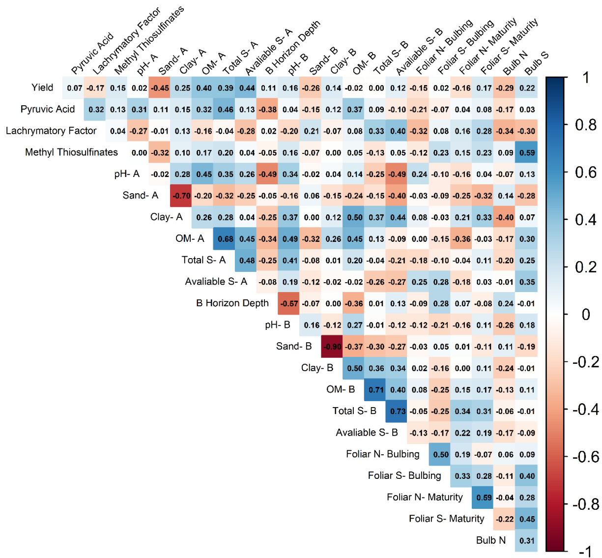
Supplemental Fig 5. Field 4 correlation table.
