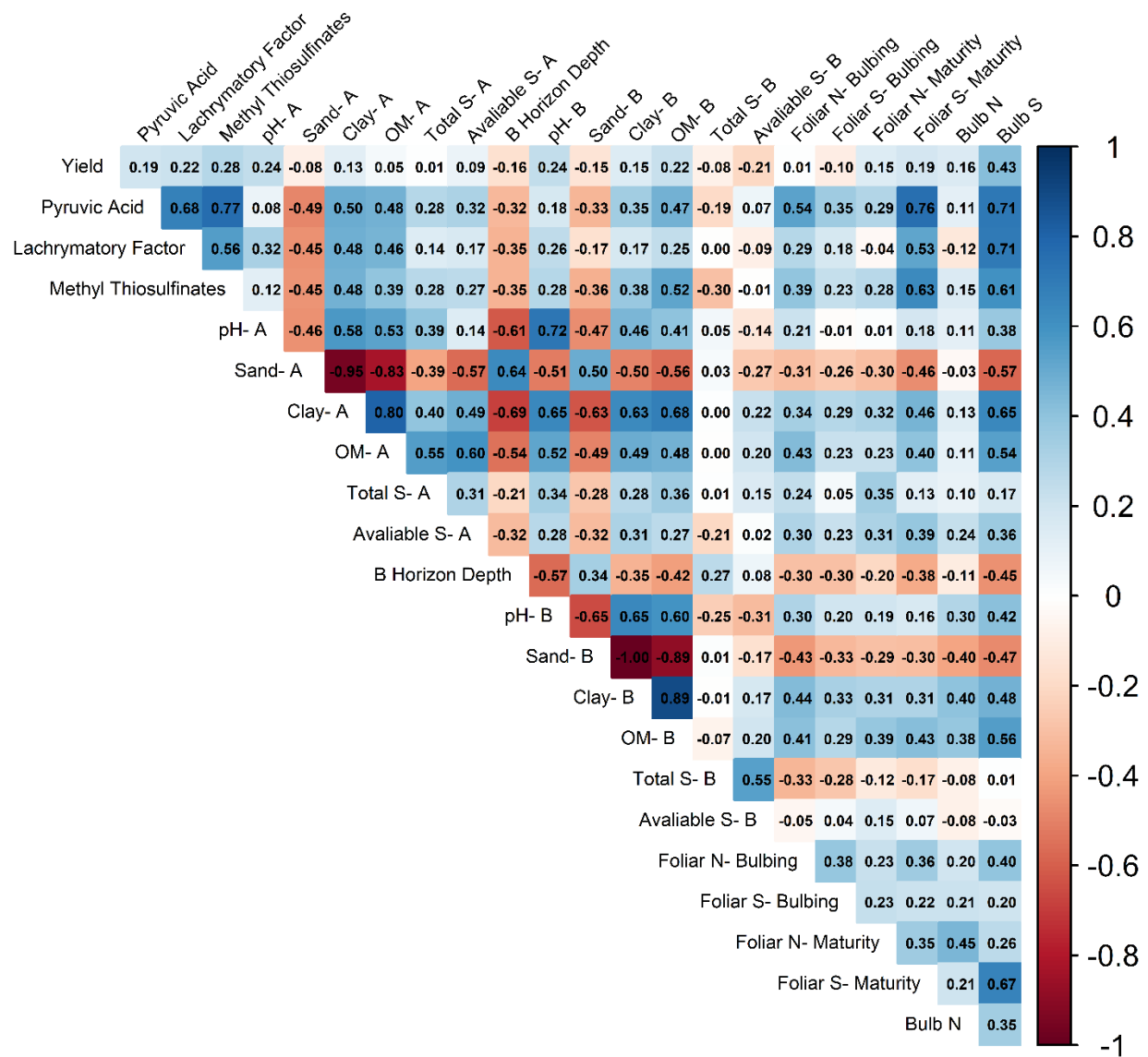
Supplemental Fig 1. Field 1 2020 correlation table.
