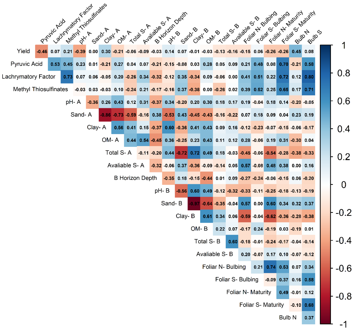
Supplemental Fig 6. Correlation table for all site-years minus the control field.
