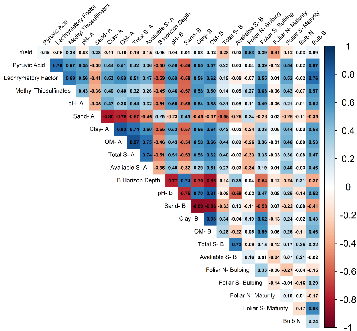
Supplemental Fig 3. Field 2 correlation table.
