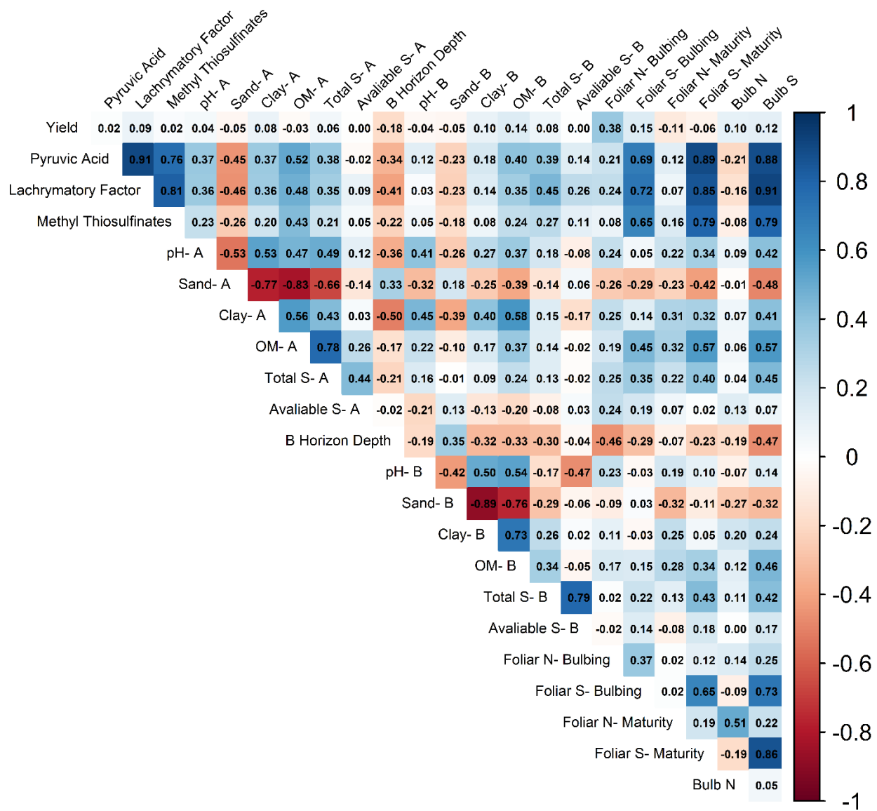
Supplemental Fig 2. Field 1 2021 correlation table.
