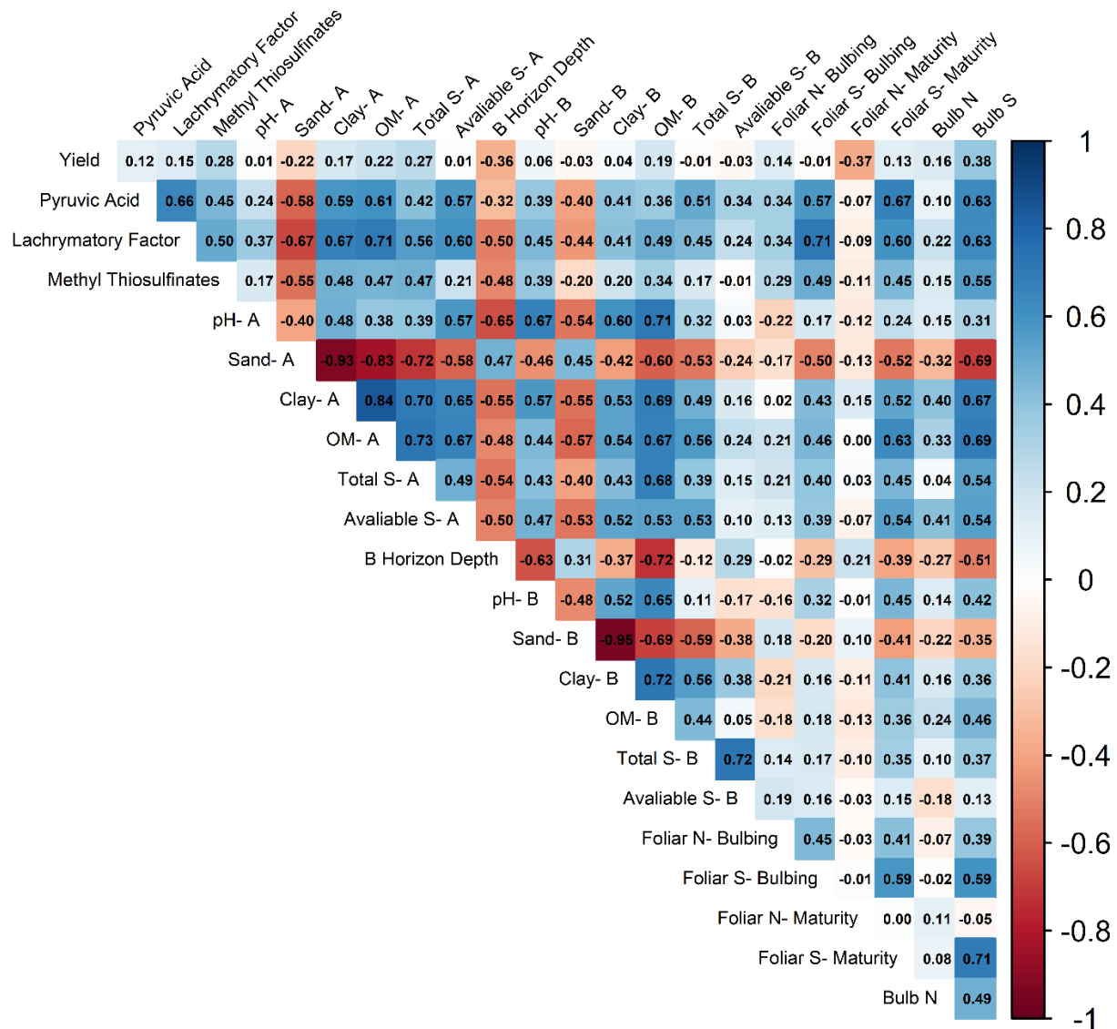
Supplemental Fig 4. Field 3 correlation table.
