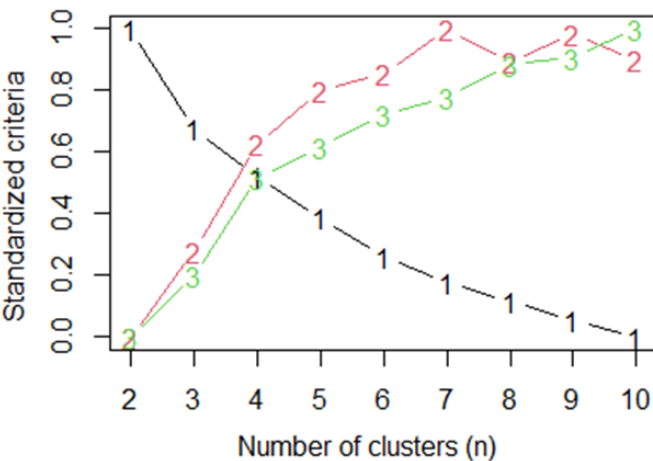
C Yearly Variation Clusters
