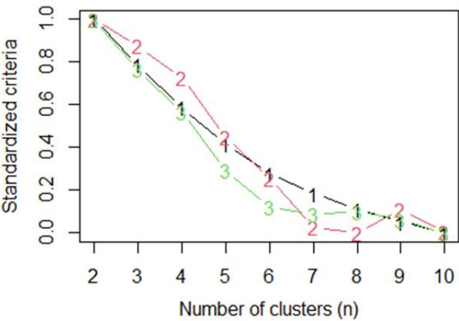
B Proportion of Yearly Citations Clusters
