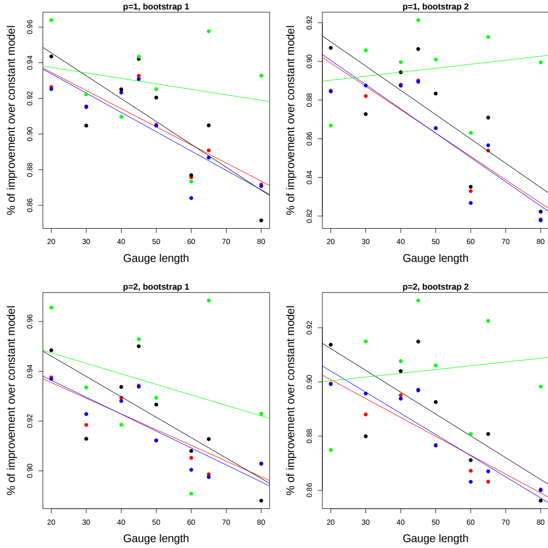
Figure 2: Scatterplot of G^*(F, \mathcal{G}) and regression line in terms of the gauge length, for the Weibull (red), 3-parameter Weibull (blue), skew normal (black) and bimodal Weibull (green).
