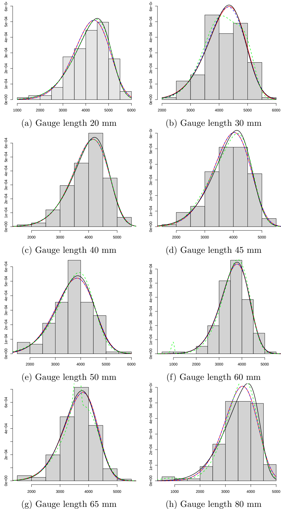
Figure 1: Histogram of failure stress data and mle-estimated Weibull (red), 3-parameter Weibull (dashed blue), skew normal (black) and bimodal Weibull (dashed green) models.
