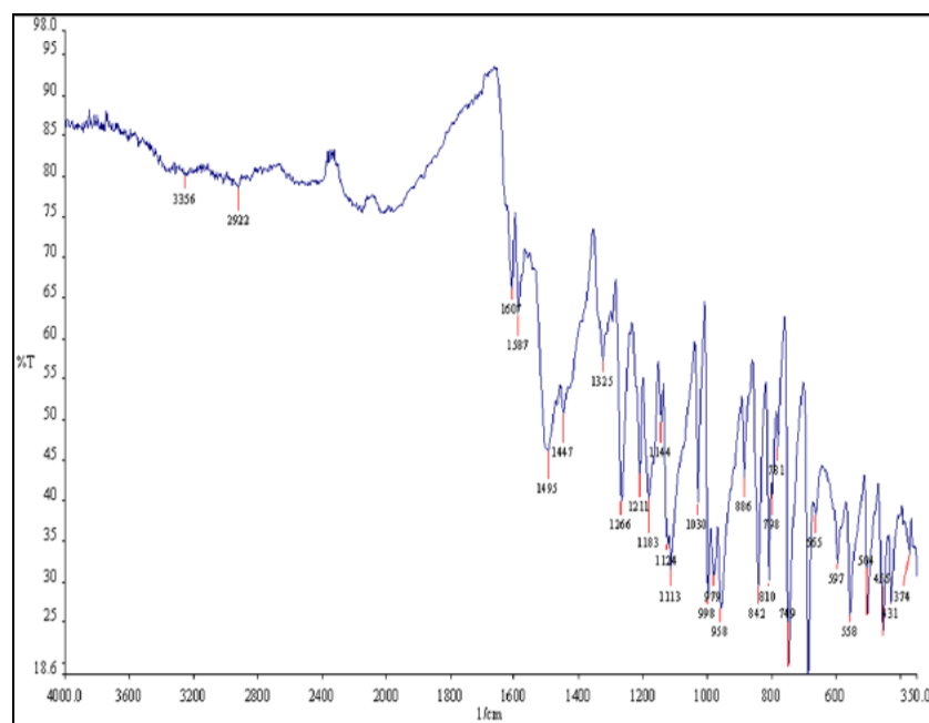
Fig S1. IR spectra of HPTO (a) Experimental and (b) theoretical
