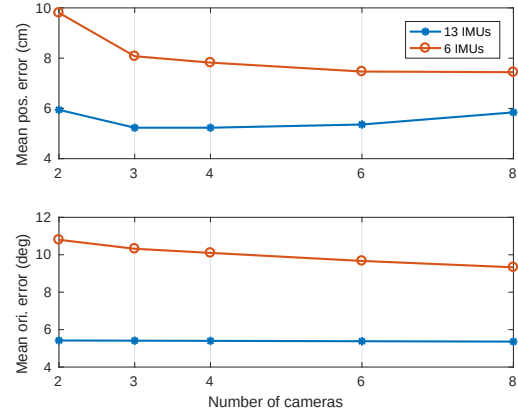
Figure 3: Position and orientation error with different sensor configurations, 13 or 6 IMUs and 2-8 cameras. Sequence: S2 - FS1, SS 1/1.
