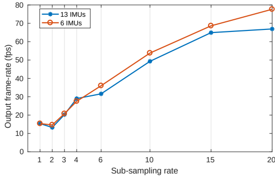
Figure 8: Output frame-rate of our solver (including detections) as a function of sub-sampling level. Sequence: S2-FS1, 4 cameras, N_o = 2 .
