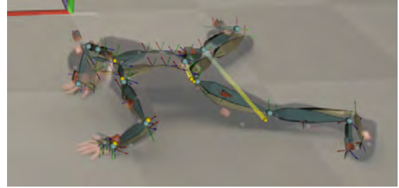
Figure 5: Solved (blue) and ground truth (yellow) skeletons overlaid on an input image showing CPM detections in yellow and the corresponding locations on the solve skeleton in blue. Note the robustness to the outlier detection on the leg. Sequence: S5, FS1.
