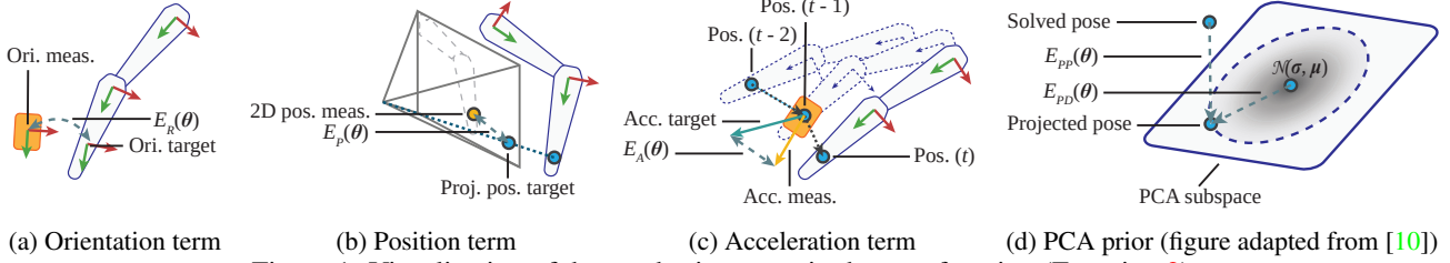
Figure 1: Visualization of data and prior terms in the cost function (Equation 2).
