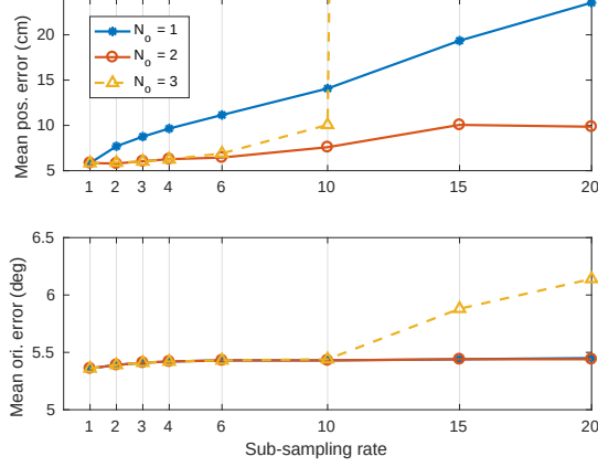
Figure 4: Position error under a range of detection sub-sampling rates using N_o \in \{1, 2, 3\} successive frames. Note that N_o = 2 yields the lowest position error across the sub-sampling range. Sequence: S2 - FS1, 13 IMUs, 8 cameras.
