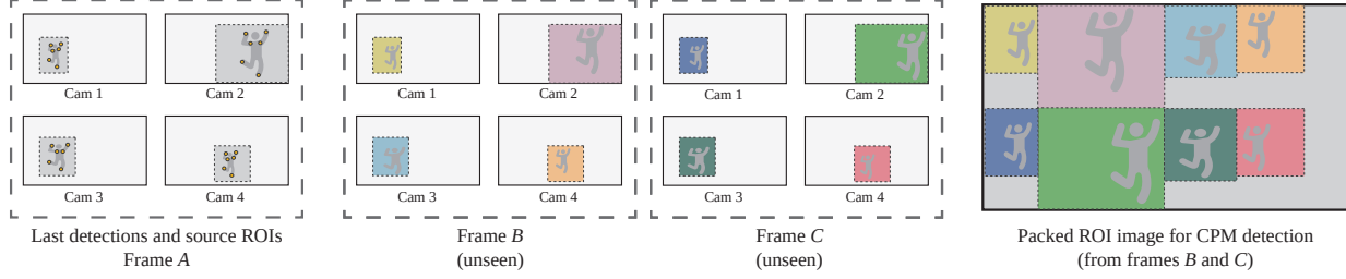
Figure 2: Visualization of the ROI packing process for efficient multi-camera/frame CPM detection.
