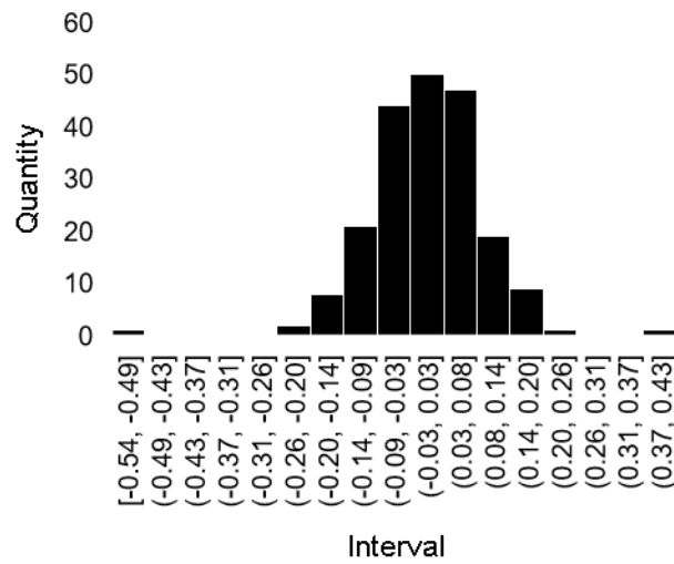
Fig. S1 Histogram of residuals (see Fig. S1)
