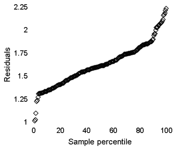
Fig. S2 Normal probability plot of residuals
