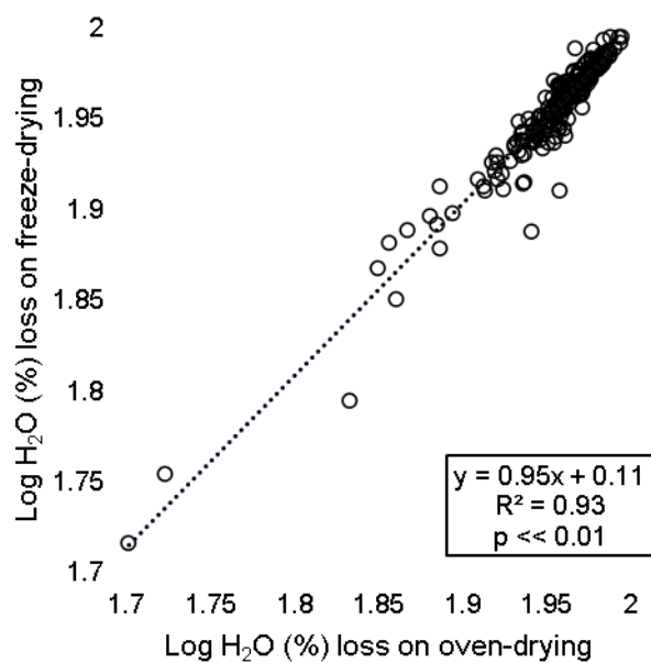
Fig. S3 Log H 2 O (%) loss on oven-drying (x-axis) vs. log H 2 O (%) loss on freeze-drying (y-axis).
