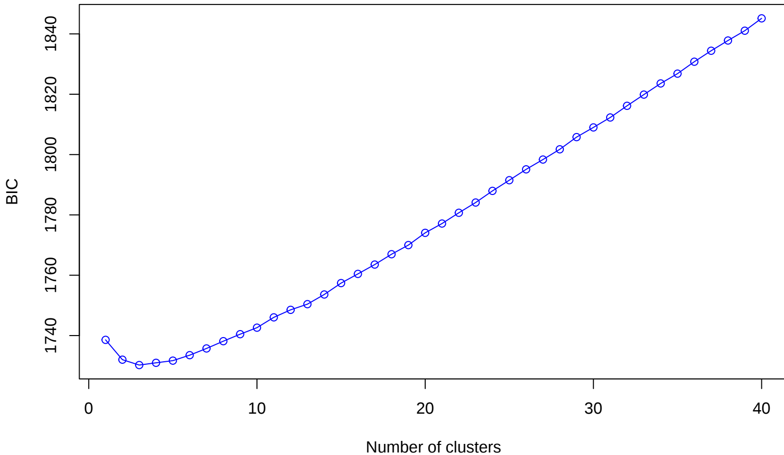
Value of BIC versus number of clusters
