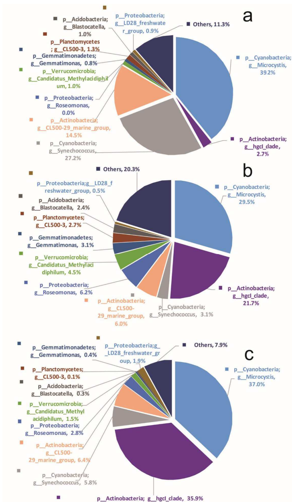
Fig. S2 Pie chart showing the relative abundance of bacteria among the V regions in water samples at the genus level. a V3, b V4, c V6
