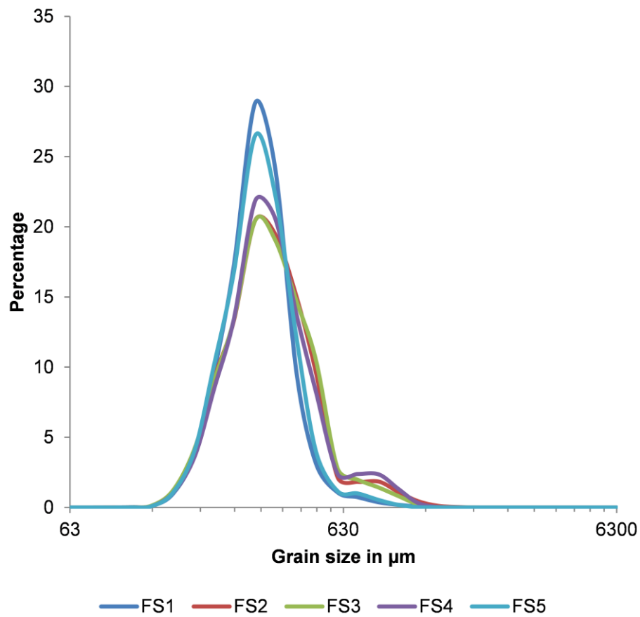
Figure 2 Grain size analysis results for five sediment samples at Falckenstein beach (FS1 – FS5). On the x-axis the grain size is displayed on a logarithmic scale. The y-axis displays the percentage share of the whole sediment sample
