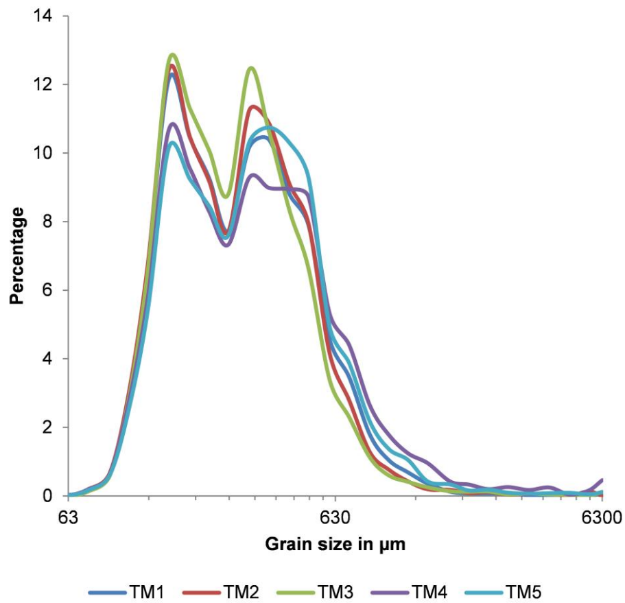
Figure 3 Grain size analysis results for five sediment samples at Tirpitzmole (TM1 –TM5). On the x-axis the grain size is displayed on a logarithmic scale. The y-axis displays the percentage share of the whole sediment sample
