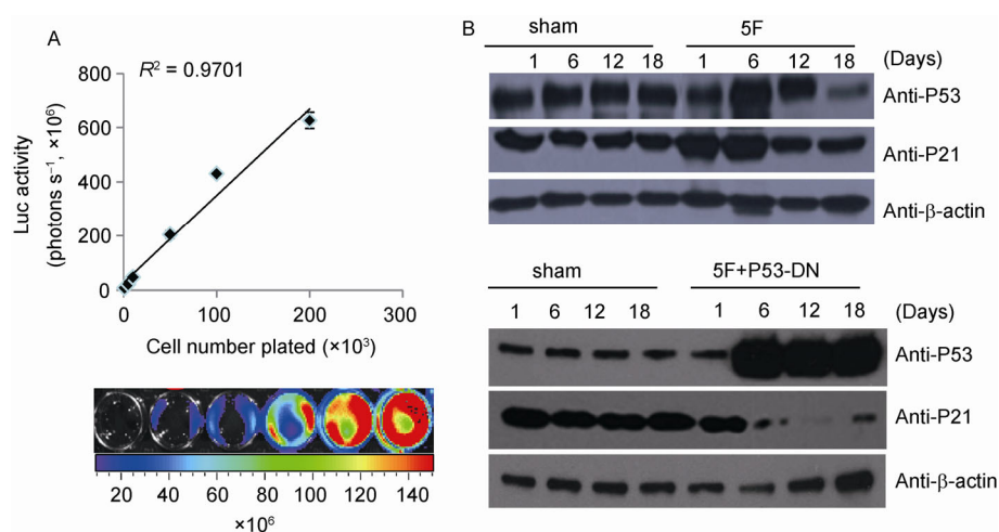
Figure S1 A, Linearity of bioluminescence vs. IMR90 cell numbers. Luc gene transduced IMR90 cells were plated in 12 well plates in different numbers. Then, cells were imaged by use of the IVIS200 imaging system. Top panel, luc activities plotted against cell number ( R^2=0.970 ). Error bars represent standard error of the mean (SEM, n=3 ). Lower panel, a representative luciferase image of the plated IMR90 cells. B, P21 is a target of p53 in the reprogramming process. Western blot analysis of p53 and p21 protein expression in 5F (upper panel) or 5F-p53-DN (lower panel) transduced IMR90 cells at indicated times.
