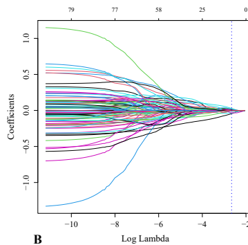
Feature selection by coefficient profile
