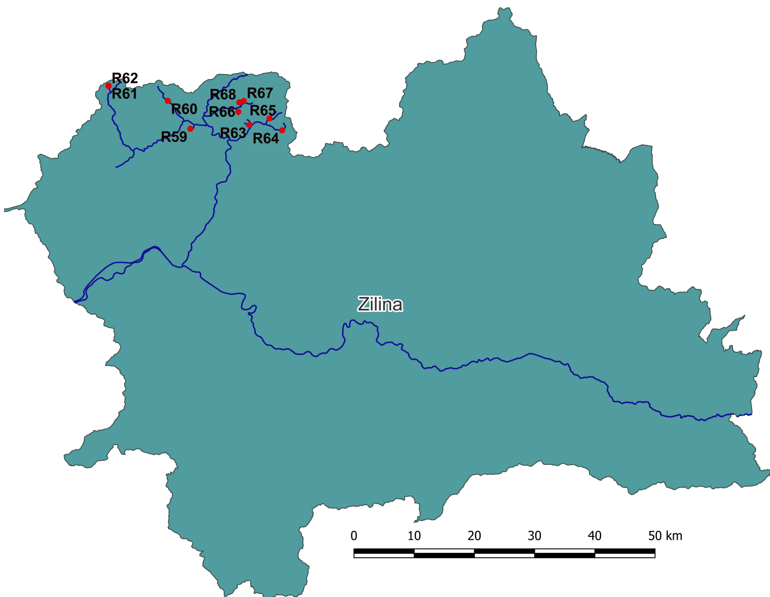
Figure S10. Distribution of sites included in the oomycete survey of forest streams in the Žilina region of Slovakia.
