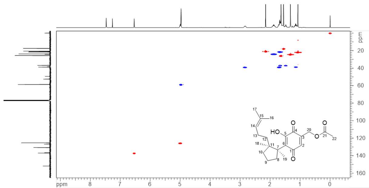
Figure S6. HSQC spectrum (400/100 MHz, CDCl 3 ) of steglichon ( 1 ).
