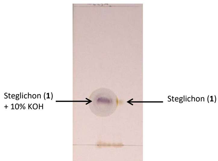
Figure S12. Color reaction of steglichon ( 1 ) on TLC with 10% KOH.
