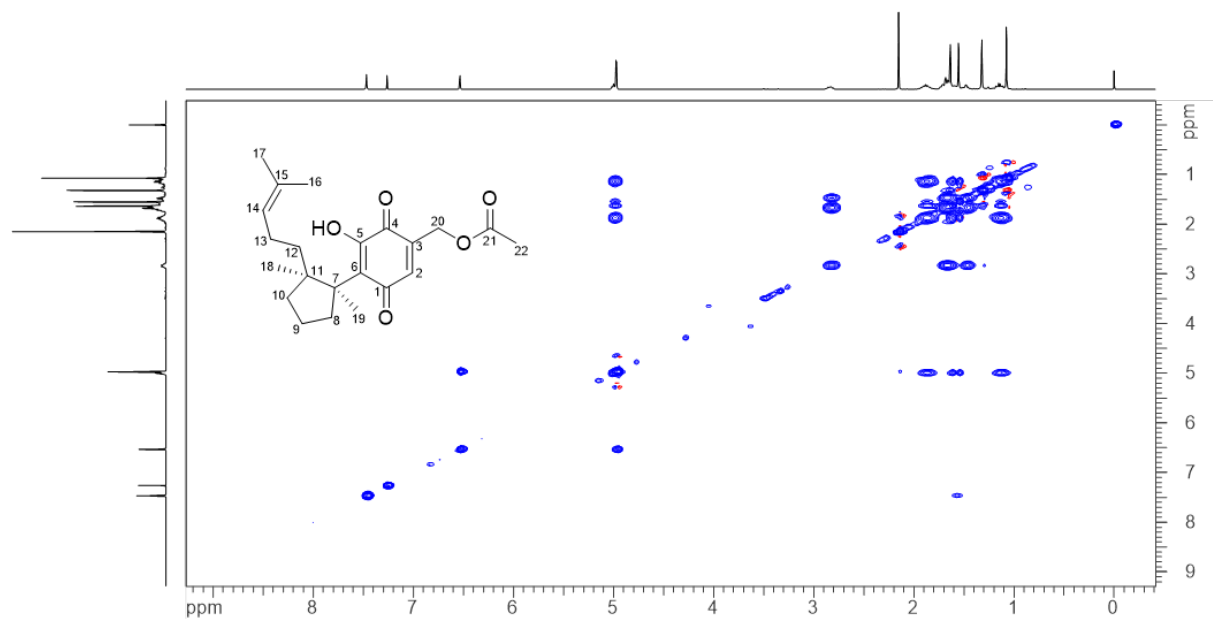
Figure S10. NOESY spectrum (400 MHz, \text{CDCl}_3 ) of steglichon ( 1 ).
