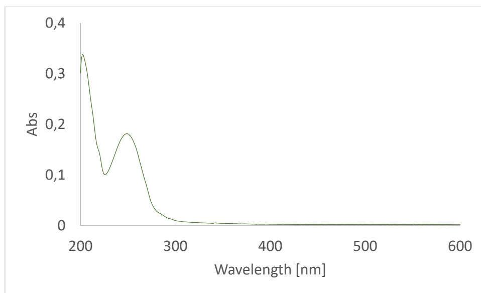
Figure S11. UV (MeOH) spectrum of steglichon ( 1 ).
