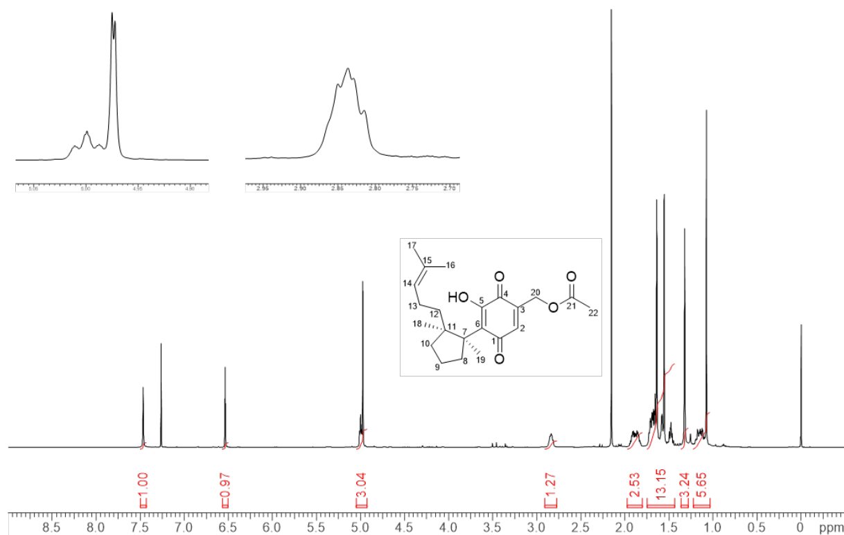
Figure S4. ^{13}\text{C} NMR spectrum (100 MHz, \text{CDCl}_3 ) of steglichon ( 1 ).
