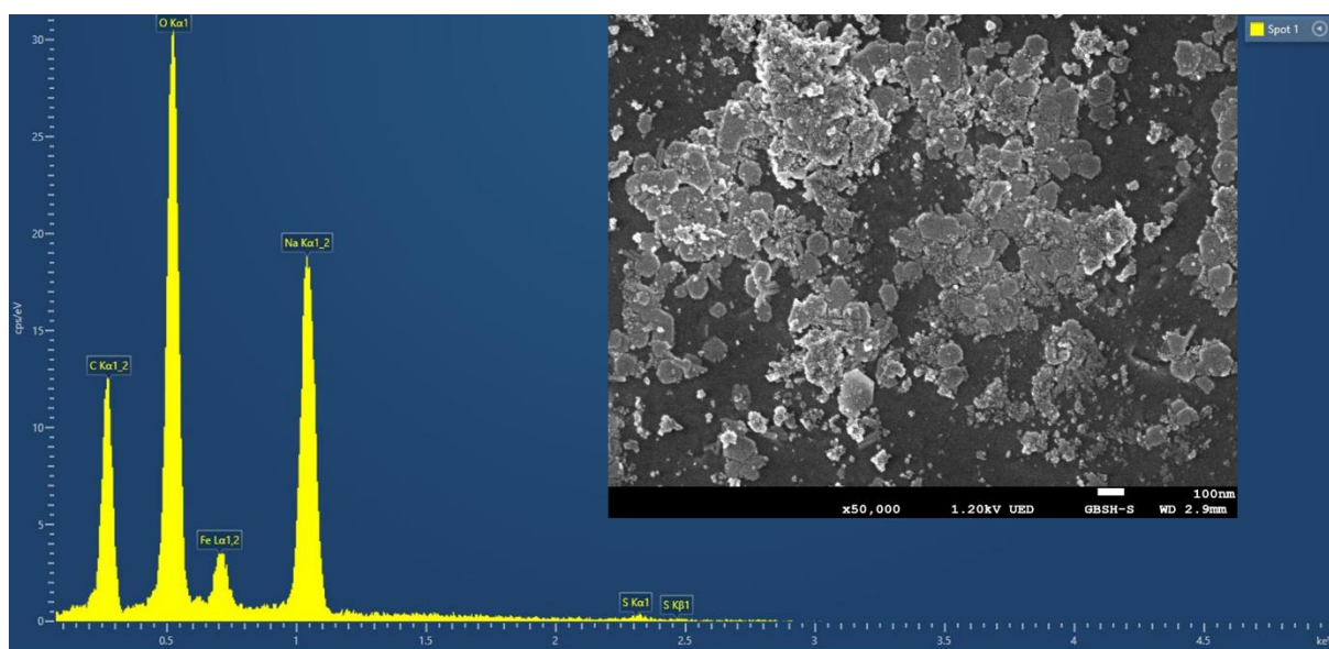
SI Fig. 1. EDS spectrum and SEM image of magnetic polymer beads
