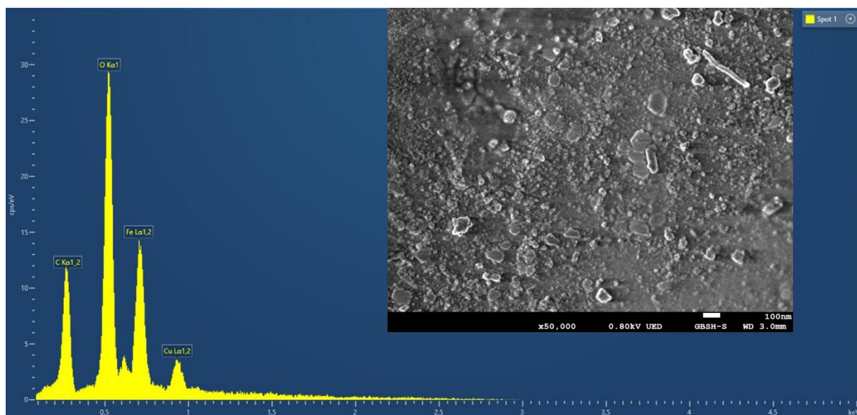
SI Fig. 3. EDS spectrum and SEM image of Cu adsorbed magnetic polymer beads
