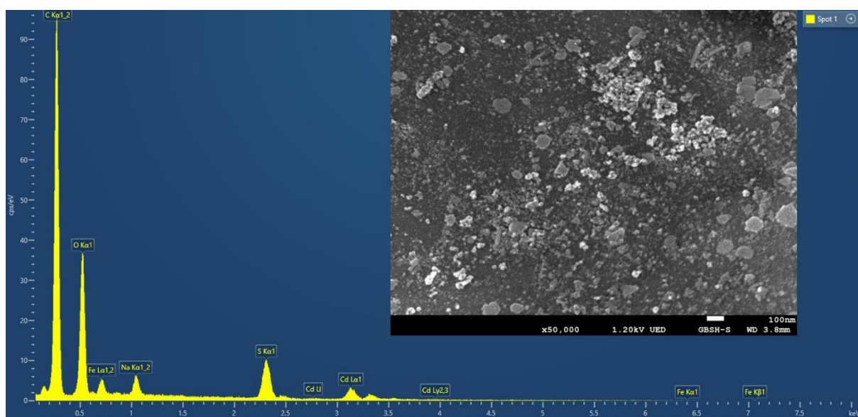
SI Fig. 2. EDS spectrum and SEM image of Cd adsorbed magnetic polymer beads
