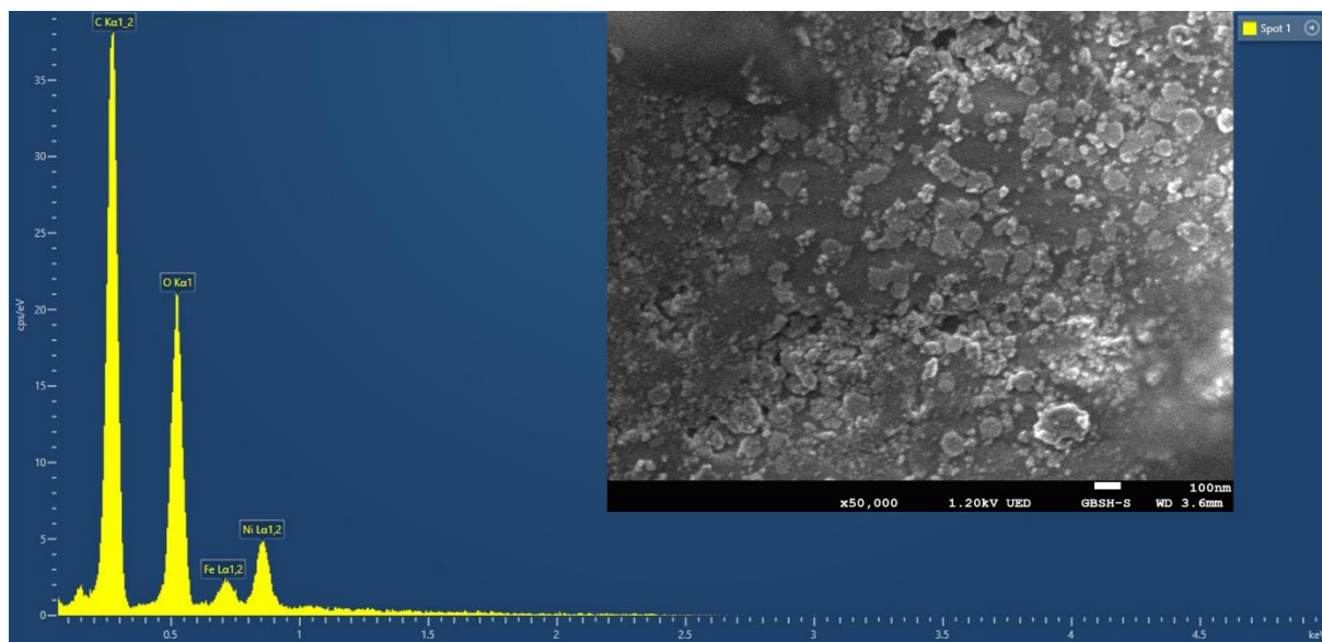
SI Fig. 5. EDS spectrum and SEM images of Ni adsorbed magnetic polymer beads
