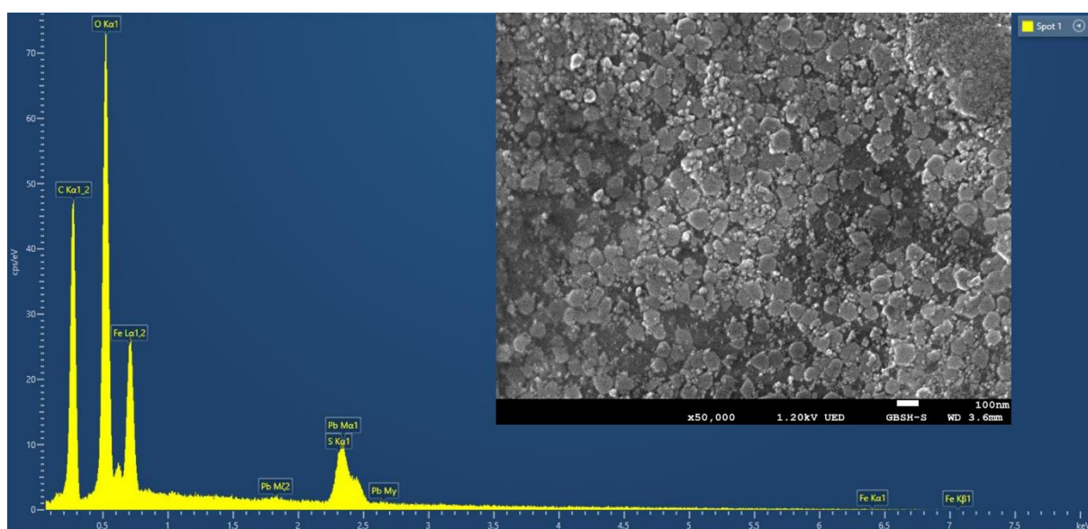
SI Fig. 4. EDS spectrum and SEM image of Pb adsorbed magnetic polymer beads
