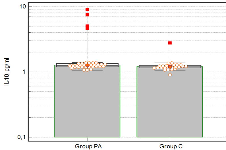
Fig. 3S The concentration of IL-10 in the blood of PA patients and healthy controls (C)
