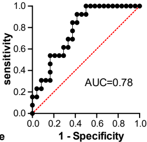
ROC curve
