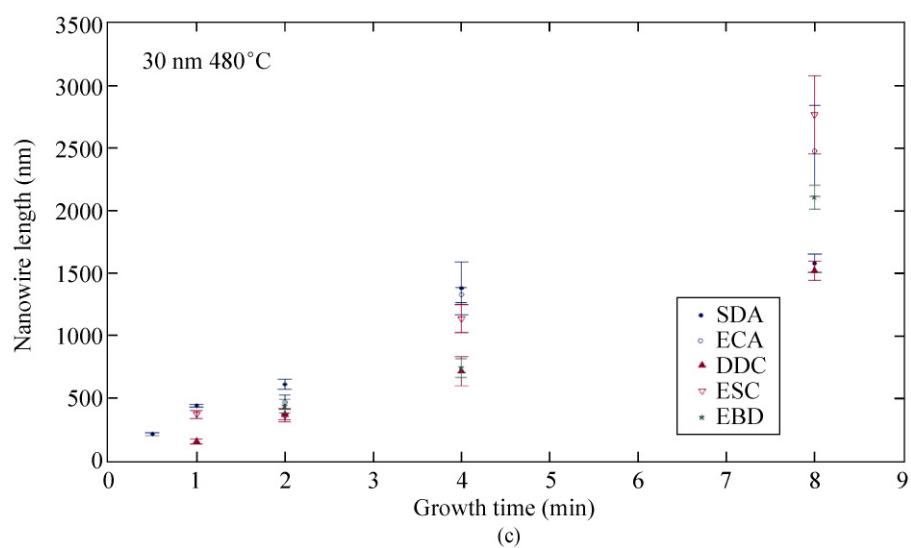
Figure S-1 Nanowire length plotted against growth time for the different 30 nm sized particle types grown at (a) 380 °C, (b) 430 °C, and (c) 480 °C
