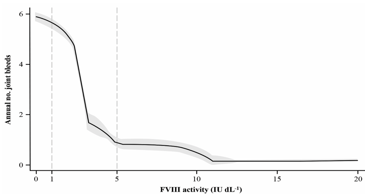
Supplementary Figure 1. Curve of AJBR with FVIII concentration change.
