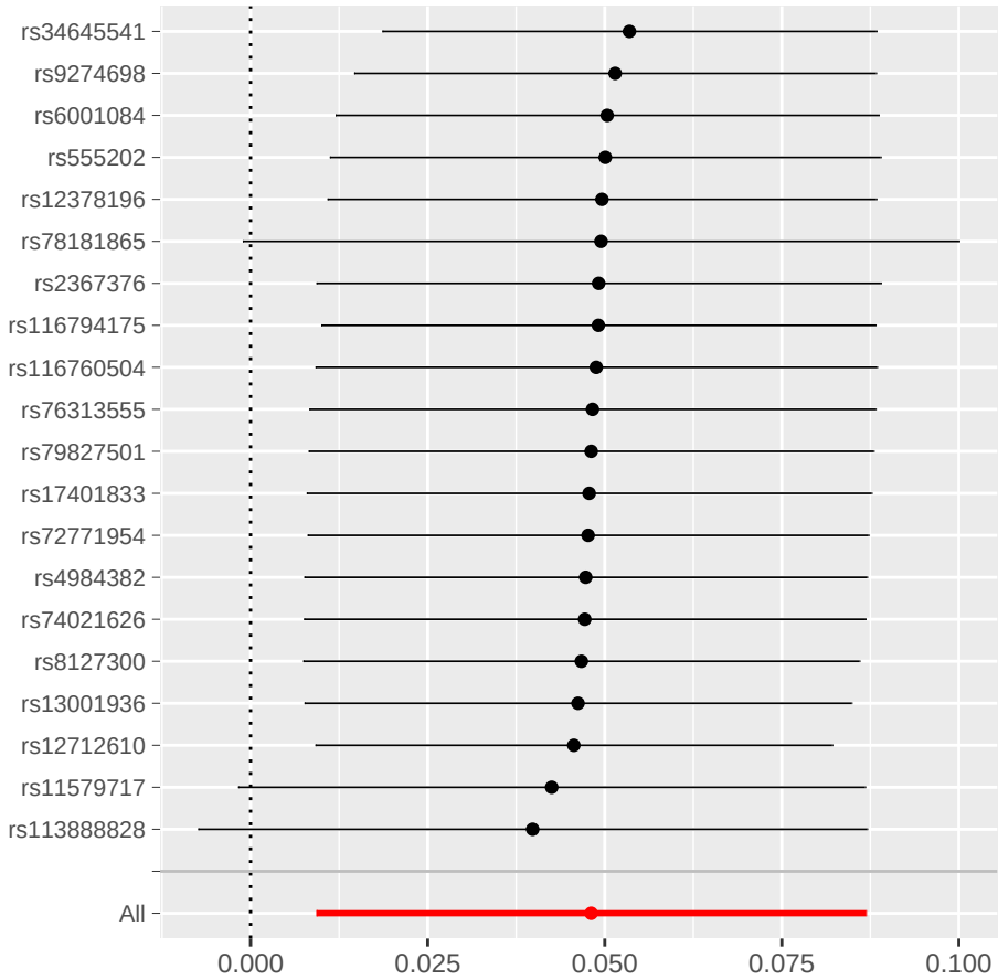
MR leave-one-out sensitivity analysis for 'CD28+ CD45RA+ CD8dim T cell %CD8dim T cell' on 'outcome'
