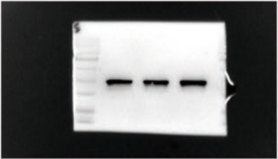
\beta -actin
