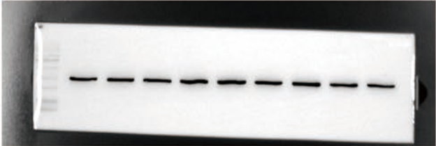
\beta -actin
