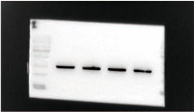
\beta -actin
