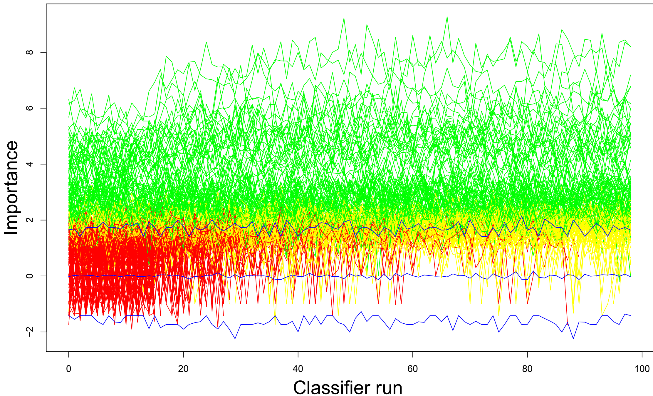
Variable Importance History Plot
