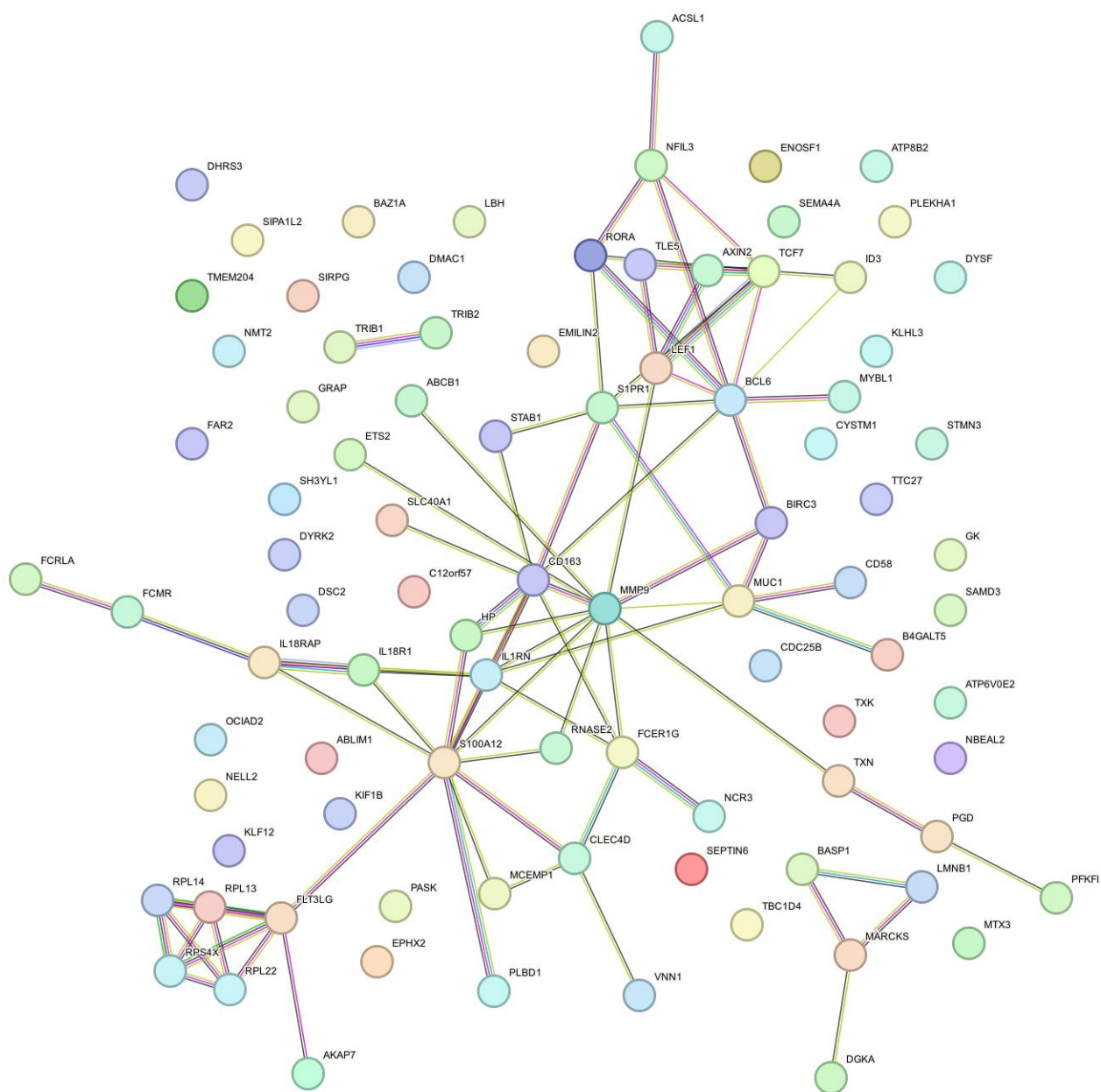
Fig. S6. Protein–protein interaction (PPI) network of validated DEGs.
