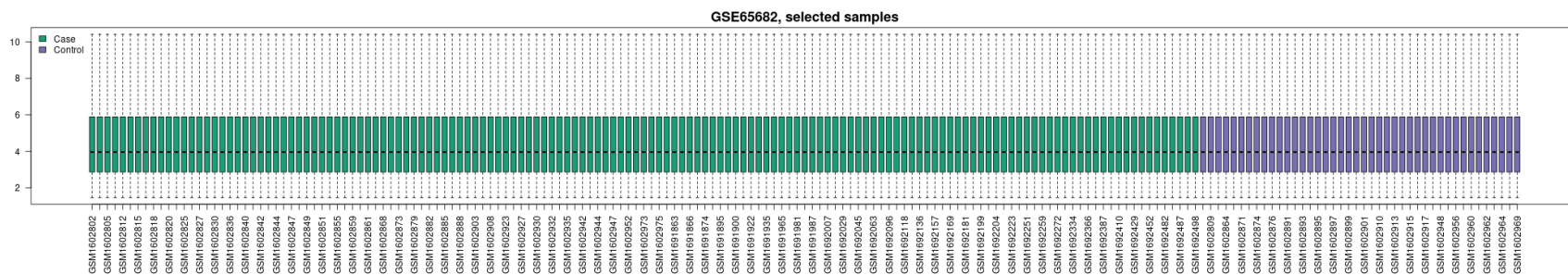
Fig. S4. Box plot visualization of normalized gene expression values comparing lung infection specimens (case) and healthy control samples in the GSE65682 dataset.
