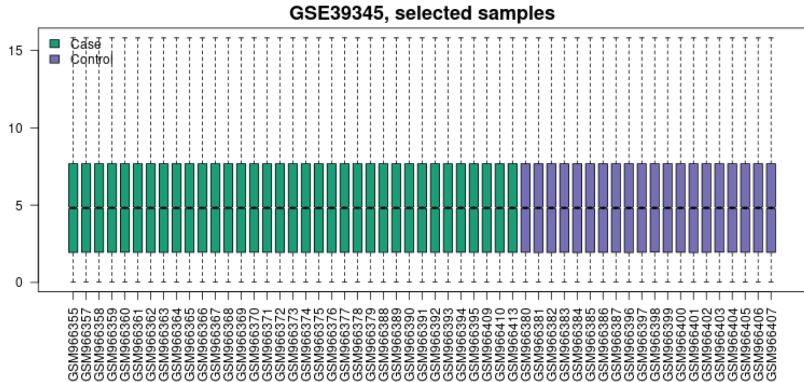
Fig. S1. Box plot visualization of normalized gene expression values comparing lung cancer specimens (case) and healthy control samples in the GSE39345 dataset.
