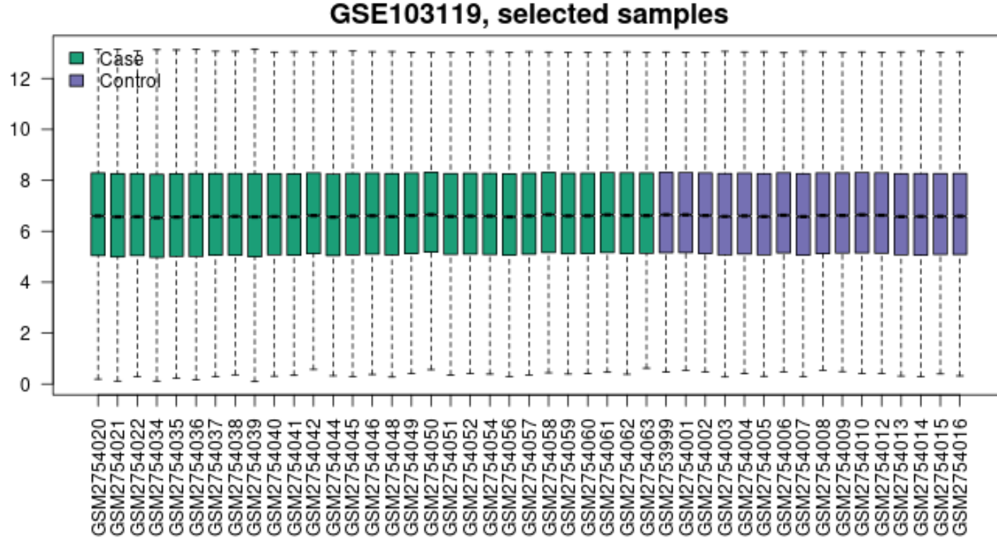
Fig. S5. Box plot visualization of normalized gene expression values comparing lung infection specimens (case) and healthy control samples in the GSE103119 dataset.
