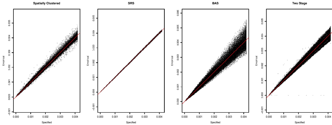
Figure A.1: Further results of simulation study. Empirical observed versus specified inclusion probabilities for four different random number generators. A) Spatial clustering (this manuscript), B) simple random sampling (SRS), C) BAS, and D) the two-stage sampling scheme defined in Section 4. If the empirical observed and specified inclusion probabilities agree, then exactly then all points will lay on the y = x line (red). Panel A) is a repeat of Figure 5C).
