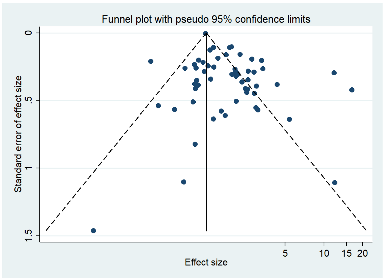
Supplementary Figure 2: Funnel plot
