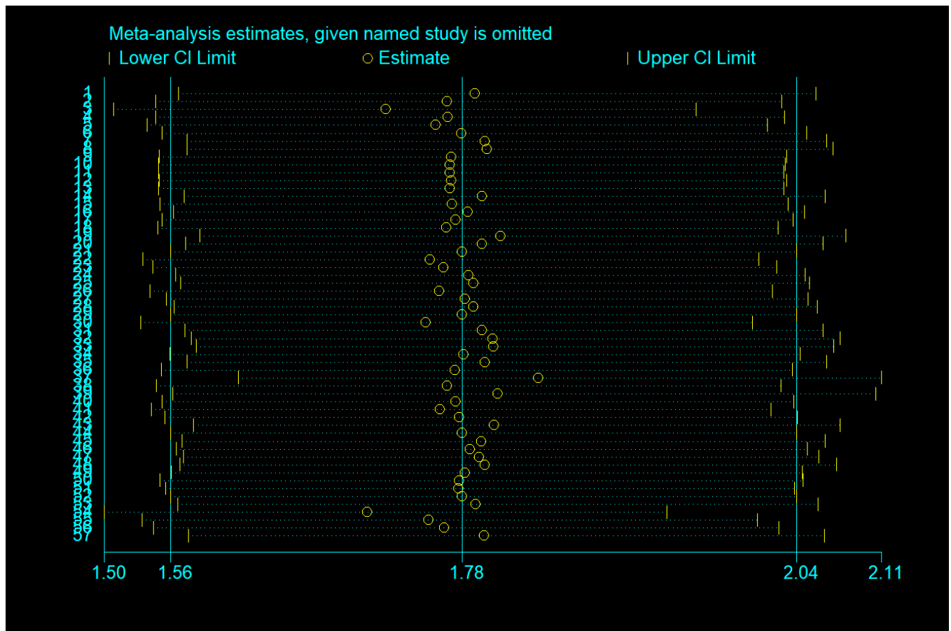
Supplementary Figure 3: Sensitivity analysis
