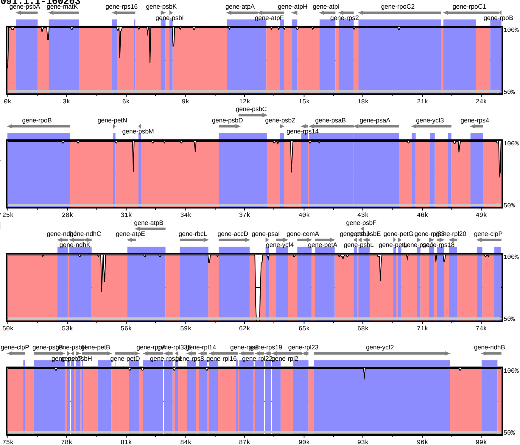
Suppl. Fig. 1: Alignment of Pyrus calleryana chloroplast to P. pyrifolia using mVista Viewer. Shown are identity scores (graph) and coding vs. non-coding regions (blue vs. red) as well as the annotation of the reference P. phaeocarpa .
