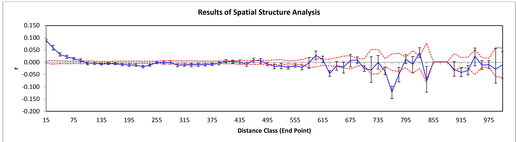
Electronic Supplementary Figure 4. Spatial autocorrelation analysis of the fox population in Great Britain for a sampling size class of 15 km. The blue line, r , is the coefficient of relatedness and the upper and lower 95% confidence intervals are shown as red dashed lines.
