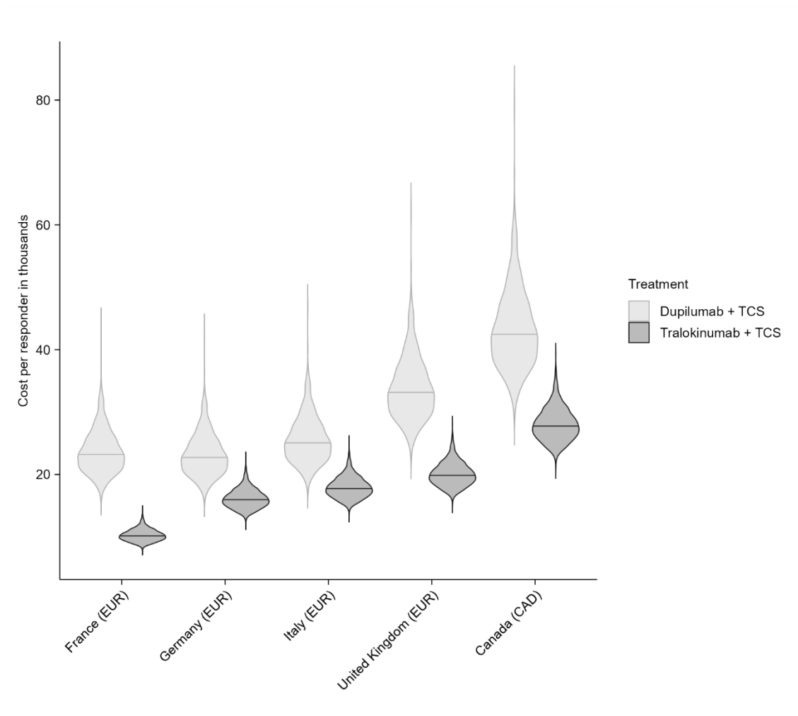
Figure S4. Violin plots for sensitivity analysis results when 40% change to Q4W (once every 4 weeks) dosing for IGA 0/1
