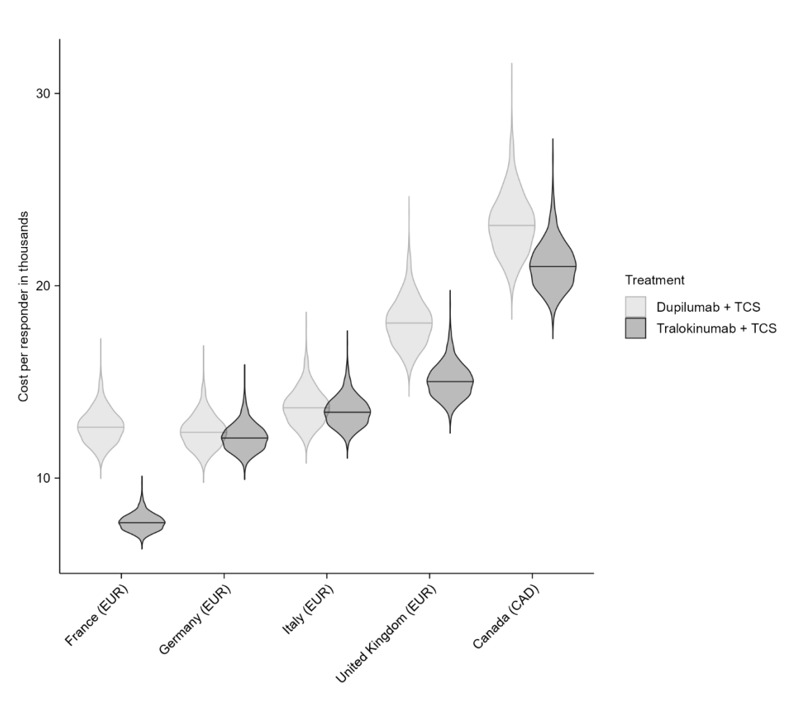
Figure S1. Violin plots for sensitivity analysis results when 10% change to Q4W (once every 4 weeks) dosing for EASI-75
