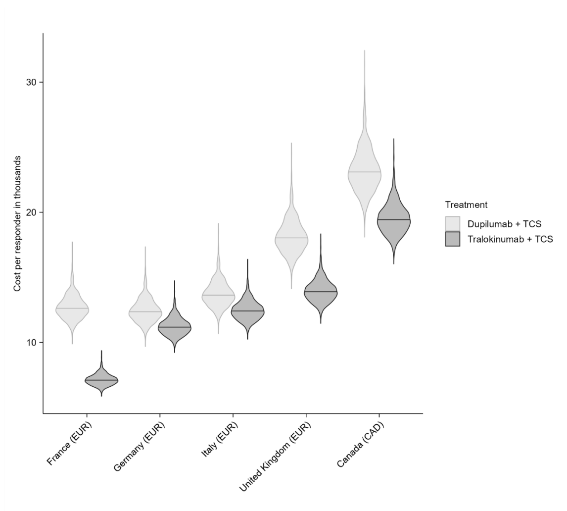
Figure S3. Violin plots for sensitivity analysis results when 40% change to Q4W (once every 4 weeks) dosing for EASI-75
