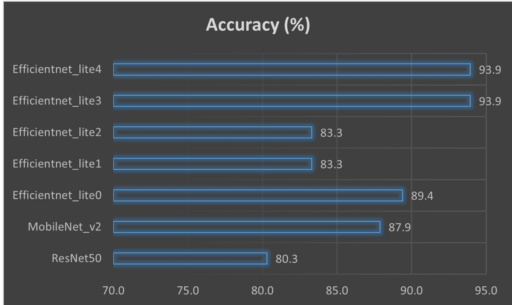
Supplemental Fig 3: Accuracy among the tested neural networks.
