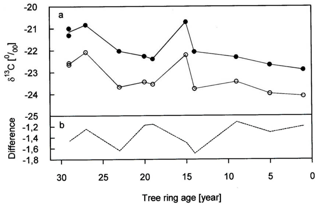
Fig. OR1. Variation of (a) \delta^{13}\text{C} from cellulose (solid symbols) and bulk wood (open symbols) and (b) the difference between both curves from the same rings (tree ring age) of five Pinus canariensis trees. Each point represents one single tree: Tree 1: tree ring age 29 and 5; Tree 2: tree ring age 29 and 15; Tree 3: tree ring age 20, 19, and 1; Tree 4: tree ring age 27 and 9; Tree 5: tree ring age 23 and 14.
