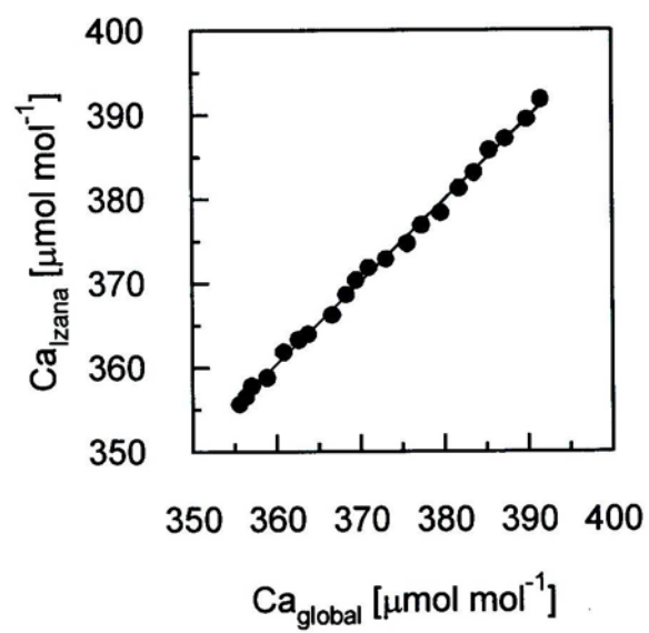
Fig. OR2. Correlation between global and local (Izaña) atmospheric CO 2 concentration obtained between 1991 and 2011. Points were fit by linear regression analysis: y=0.98x+8.8 , R^2 = 0.99 , P < 0.001
