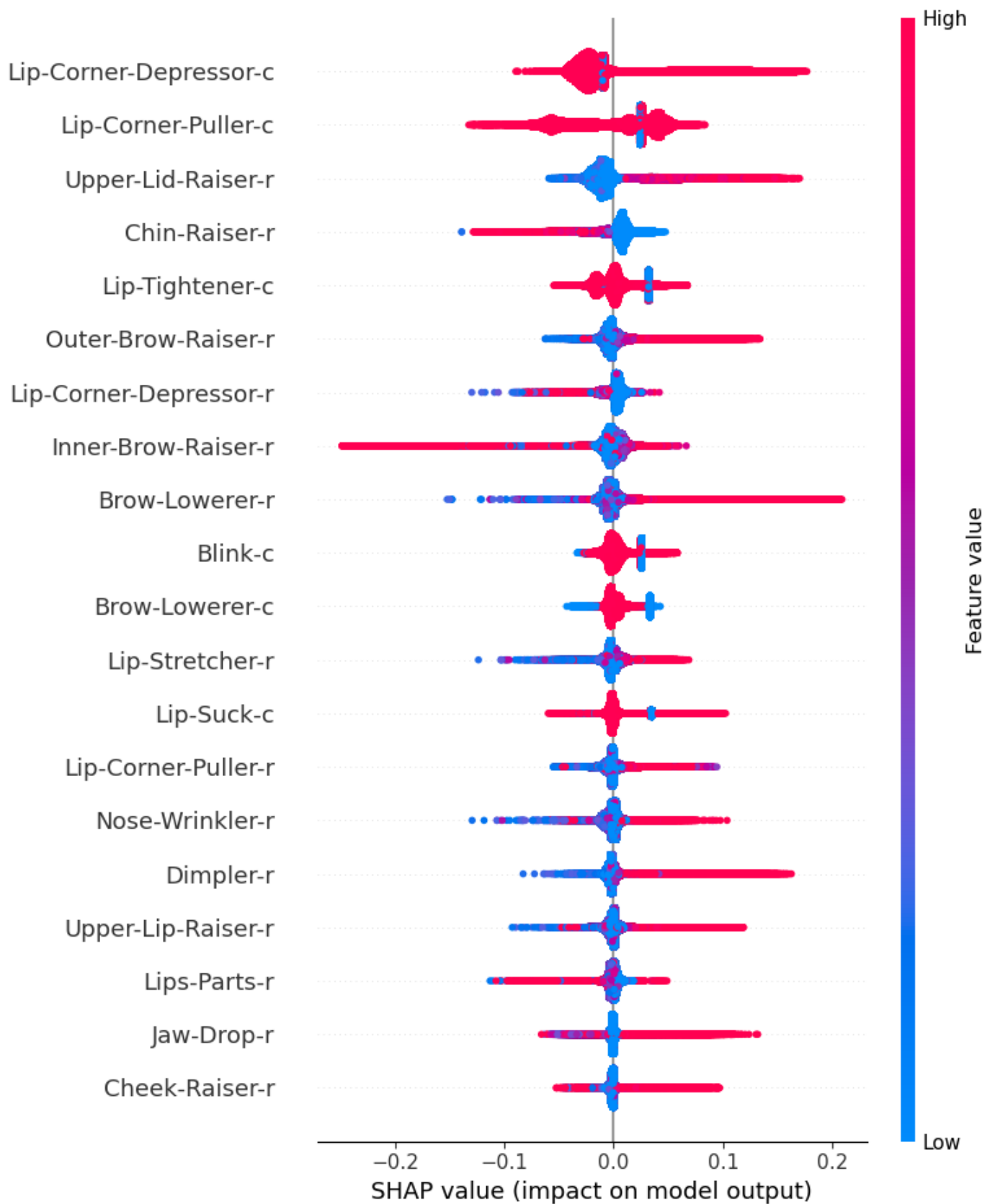
Fig. S25. Twenty most important features for AUs-Women – Iteration 5.
