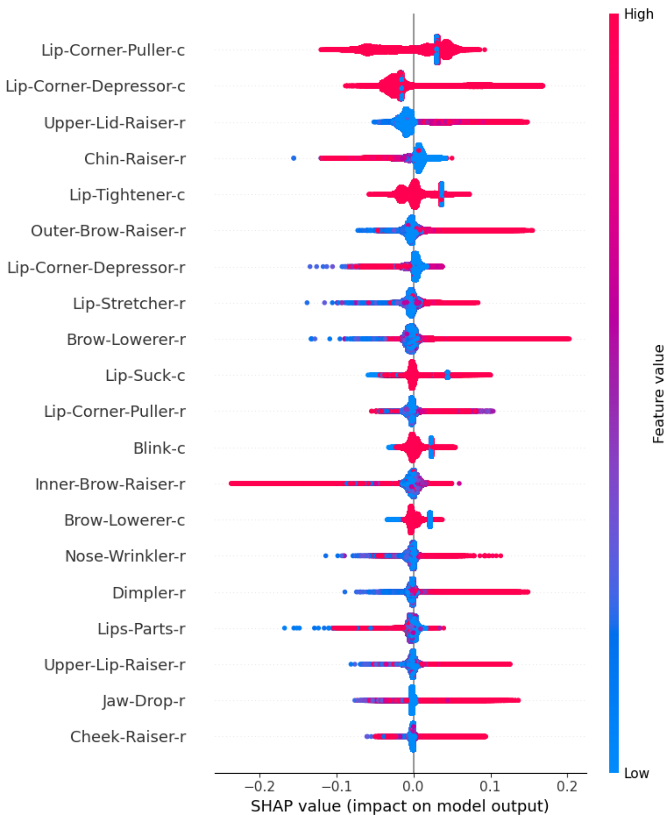
Fig. S28. Twenty most important features for AU-Weibull – Iteration 8.
