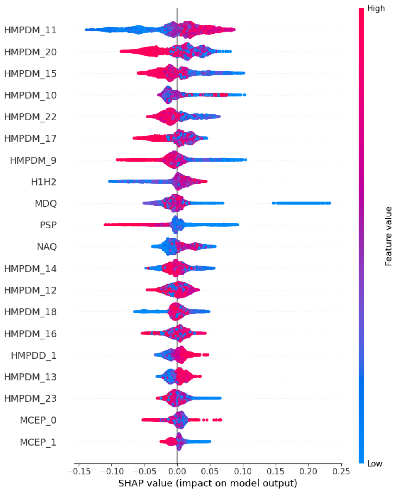
Fig. S19. Twenty most important features for Speech-Men – Iteration 9.
