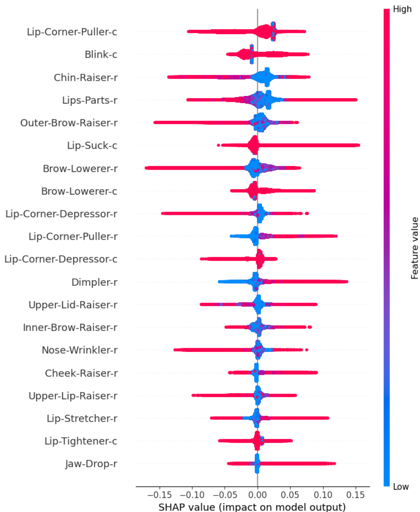
Fig. S31. Twenty most important features for AUs-Men – Iteration 1.
