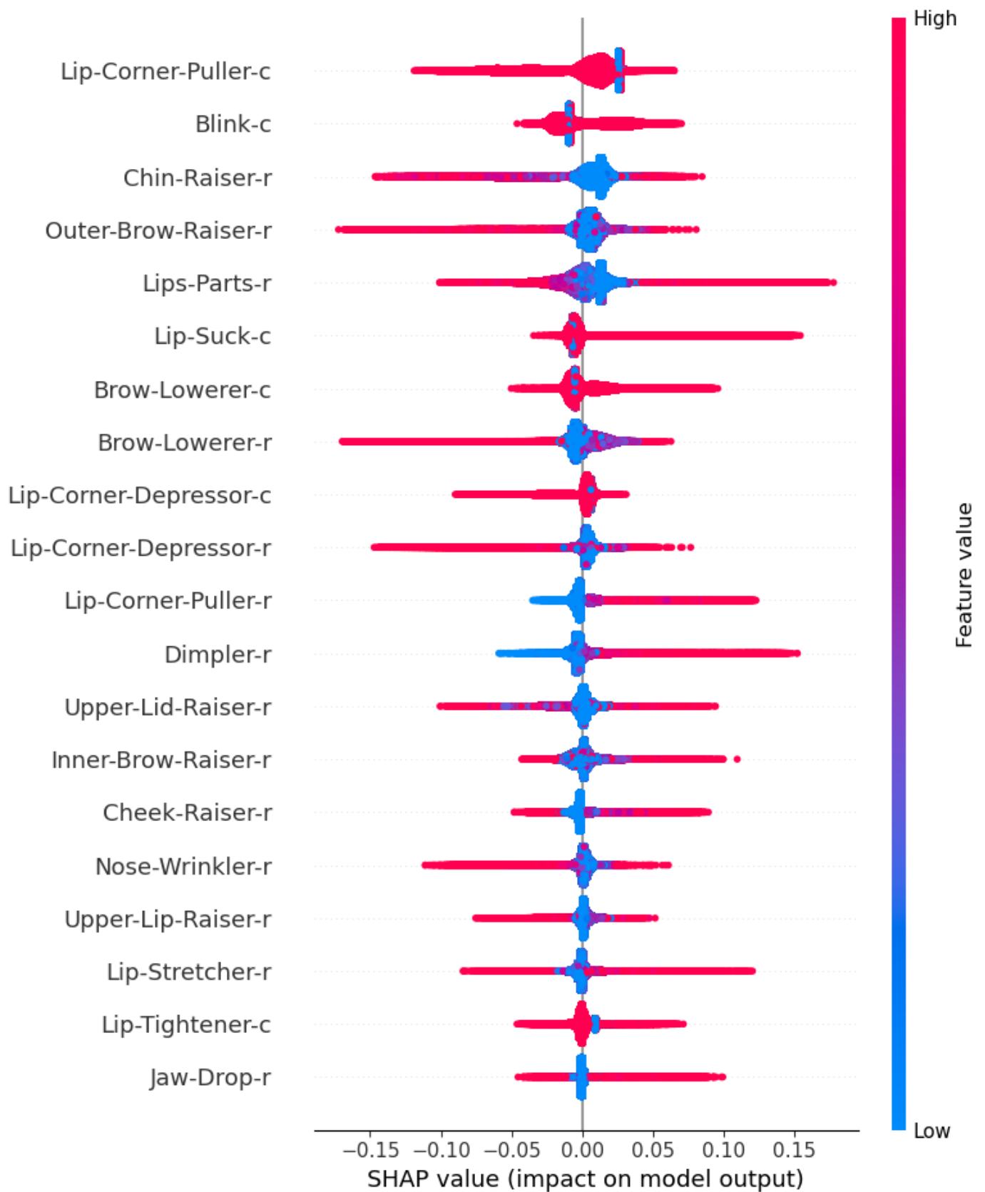
Fig. S34. Twenty most important features for AUs-Men – Iteration 4.
