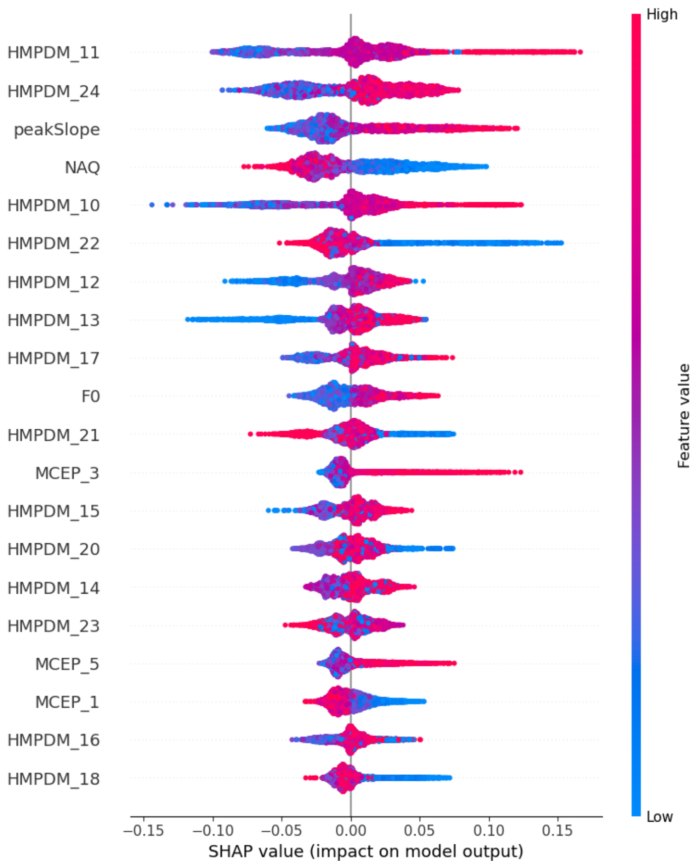
Fig. S9. Twenty most important features for Speech-Women – Iteration 9.
