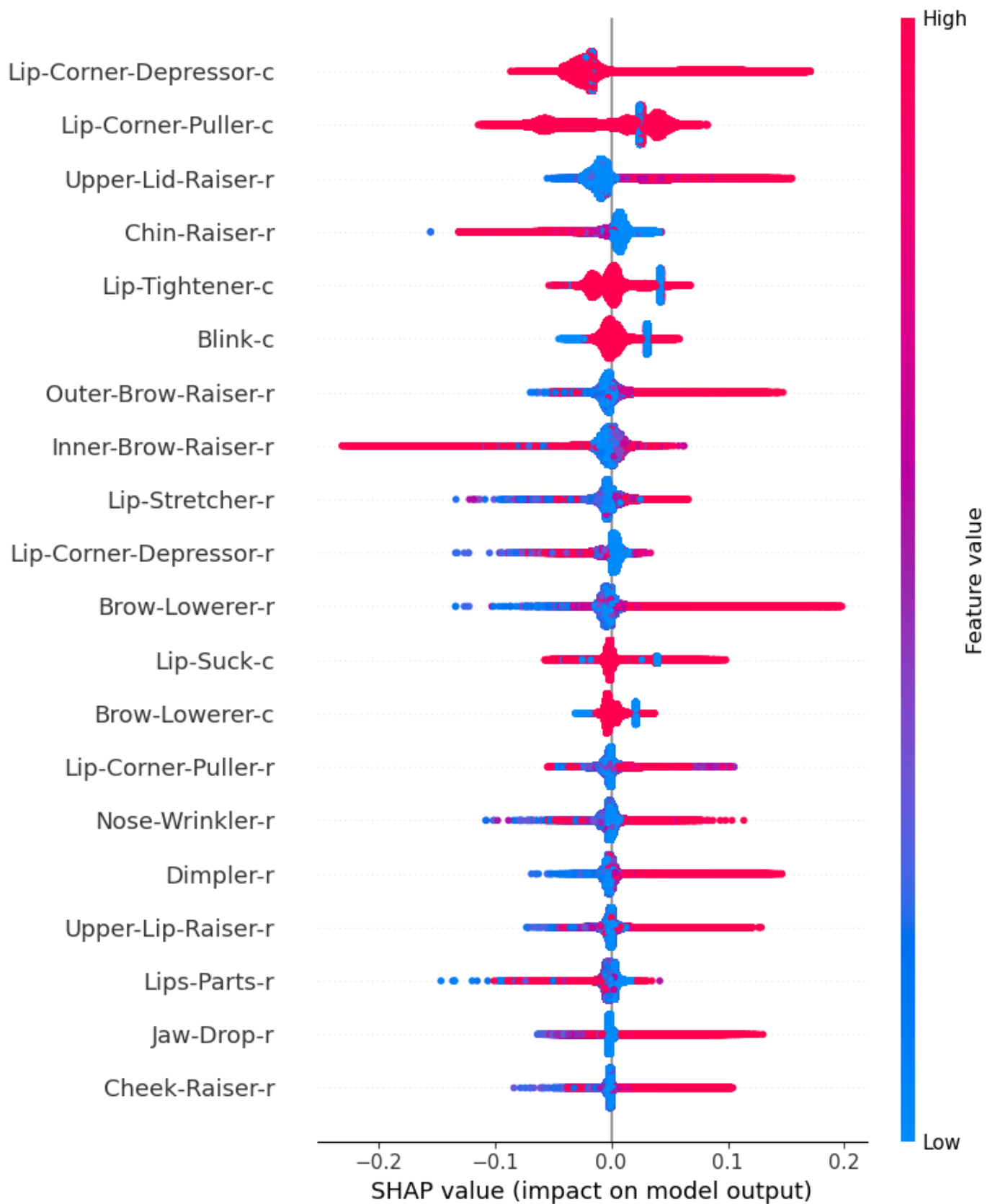
Fig. S27. Twenty most important features for AUs-Women – Iteration 7.
