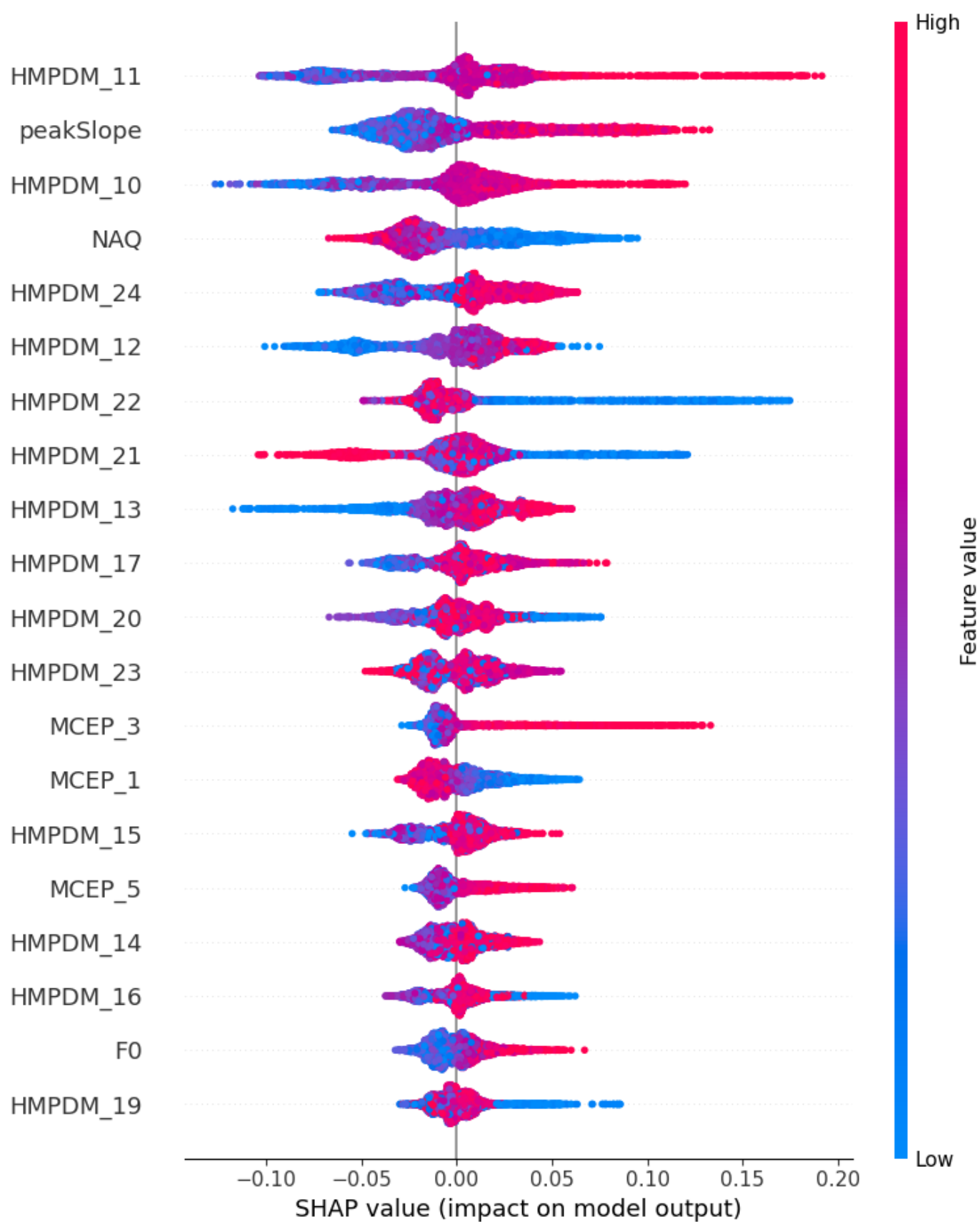
Fig. S8. Twenty most important features for Speech-Women – Iteration 8.
