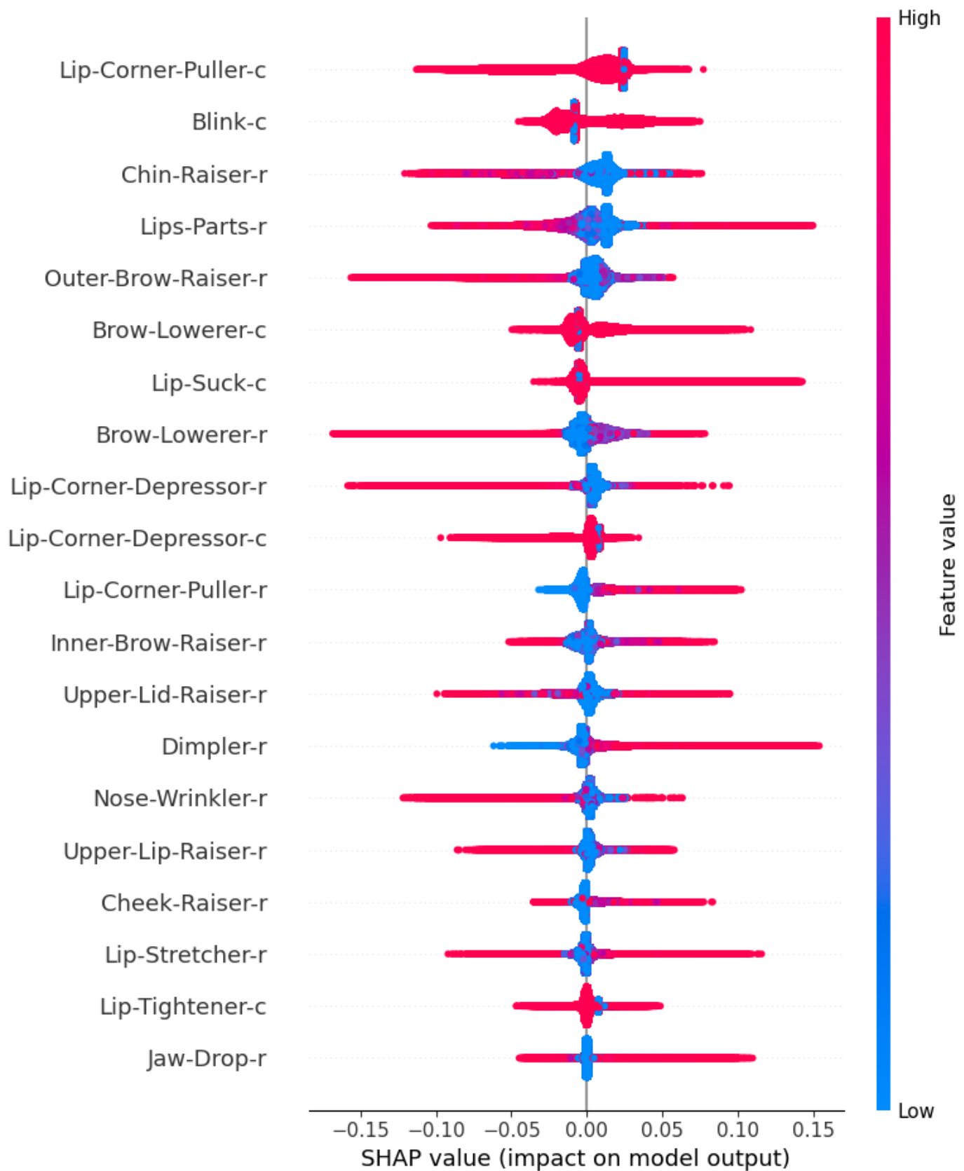
Fig. S37. Twenty most important features for AUs-Men – Iteration 7.
