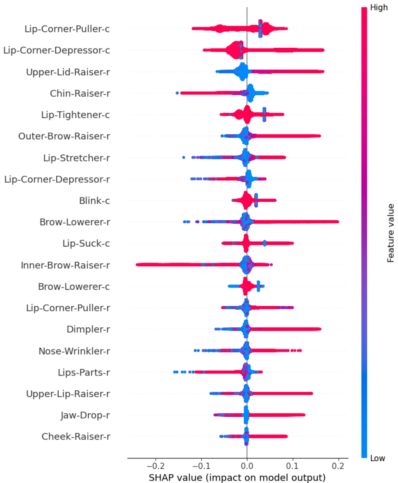
Fig. S29. Twenty most important features for AU-Weibull – Iteration 9.
