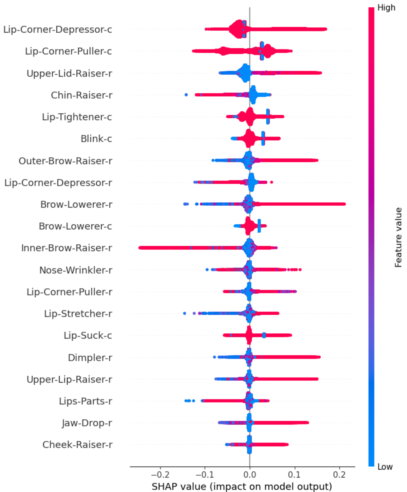
Fig. S23. Twenty most important features for AUs-Women – Iteration 3.
