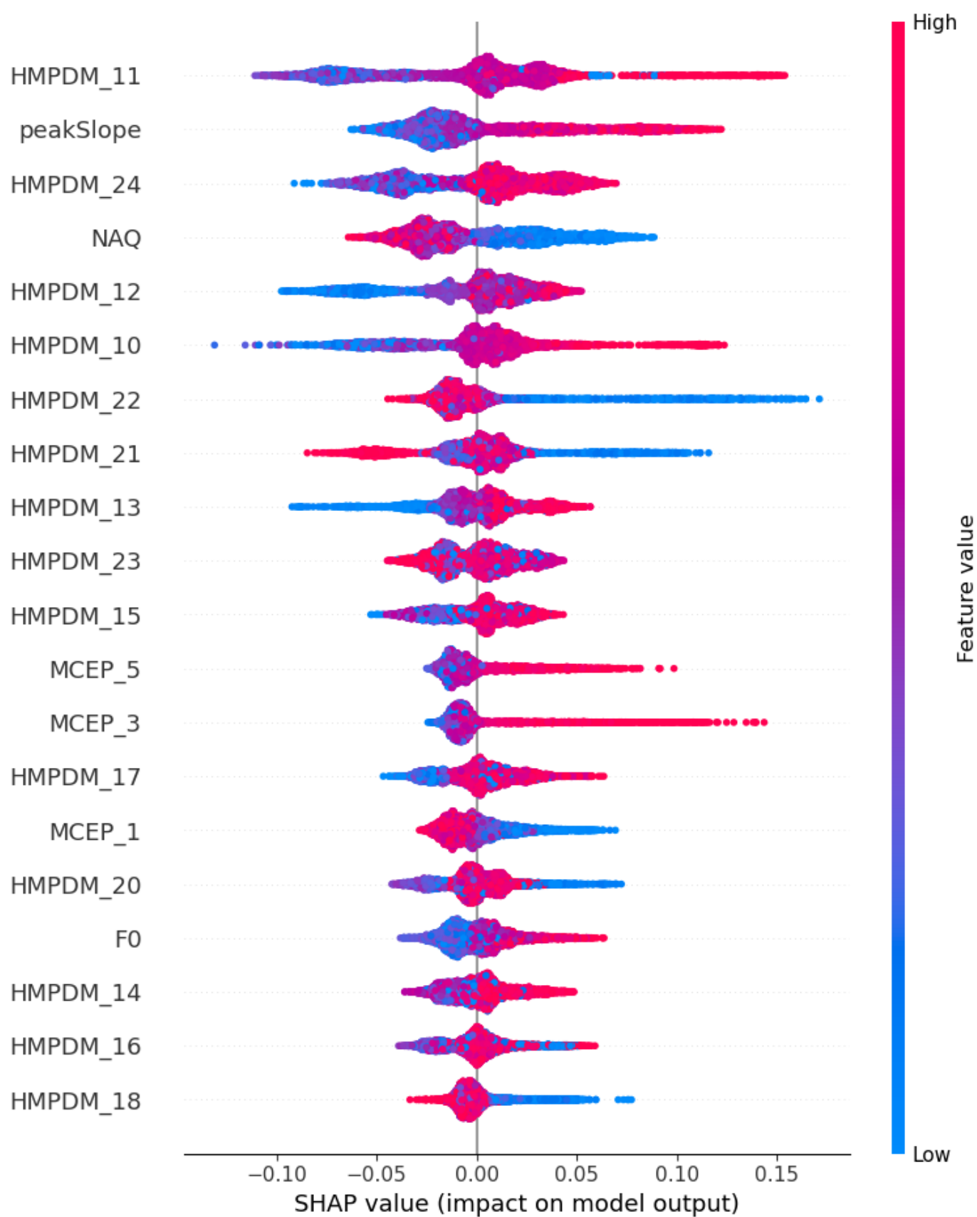
Fig. S7. Twenty most important features for Speech-Women – Iteration 7.
