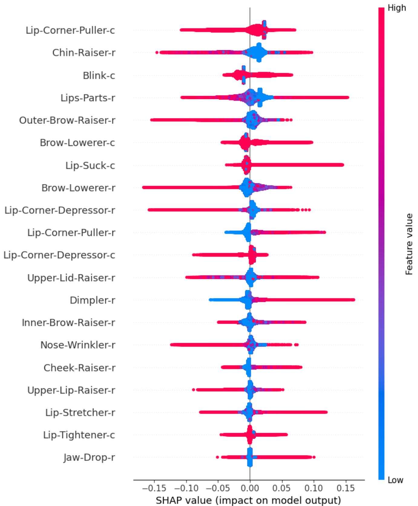
Fig. S36. Twenty most important features for AUs-Men – Iteration 6.
