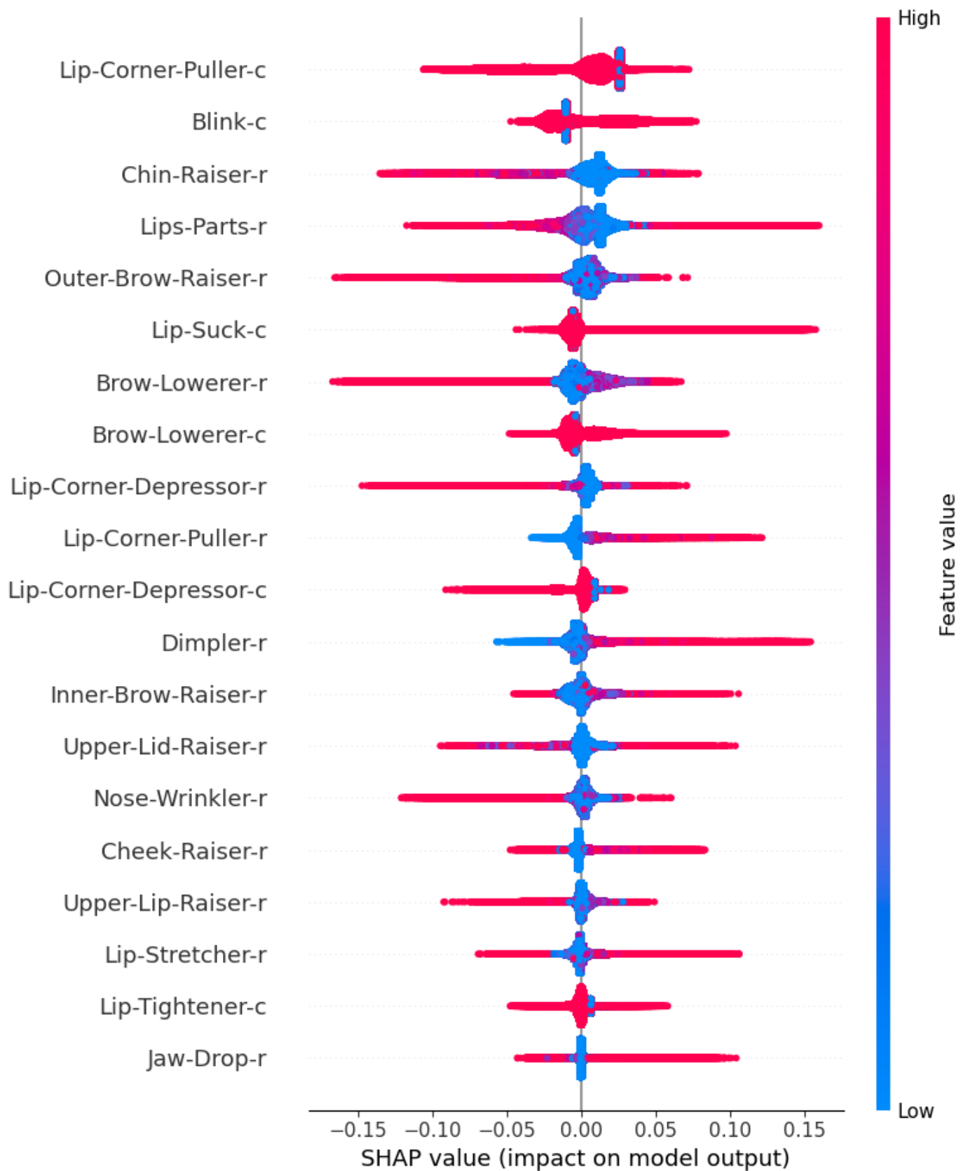
Fig. S40. Twenty most important features for AUs-Men – Iteration 10.
