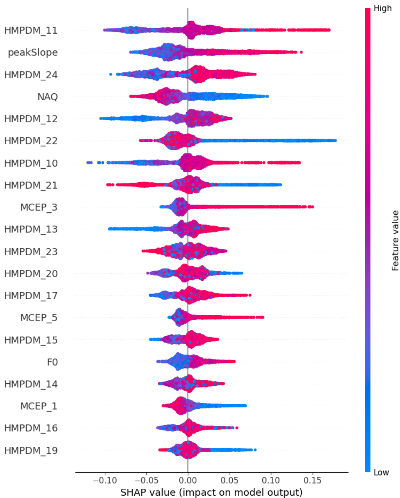
Fig. S6. Twenty most important features for Speech-Women – Iteration 6.
