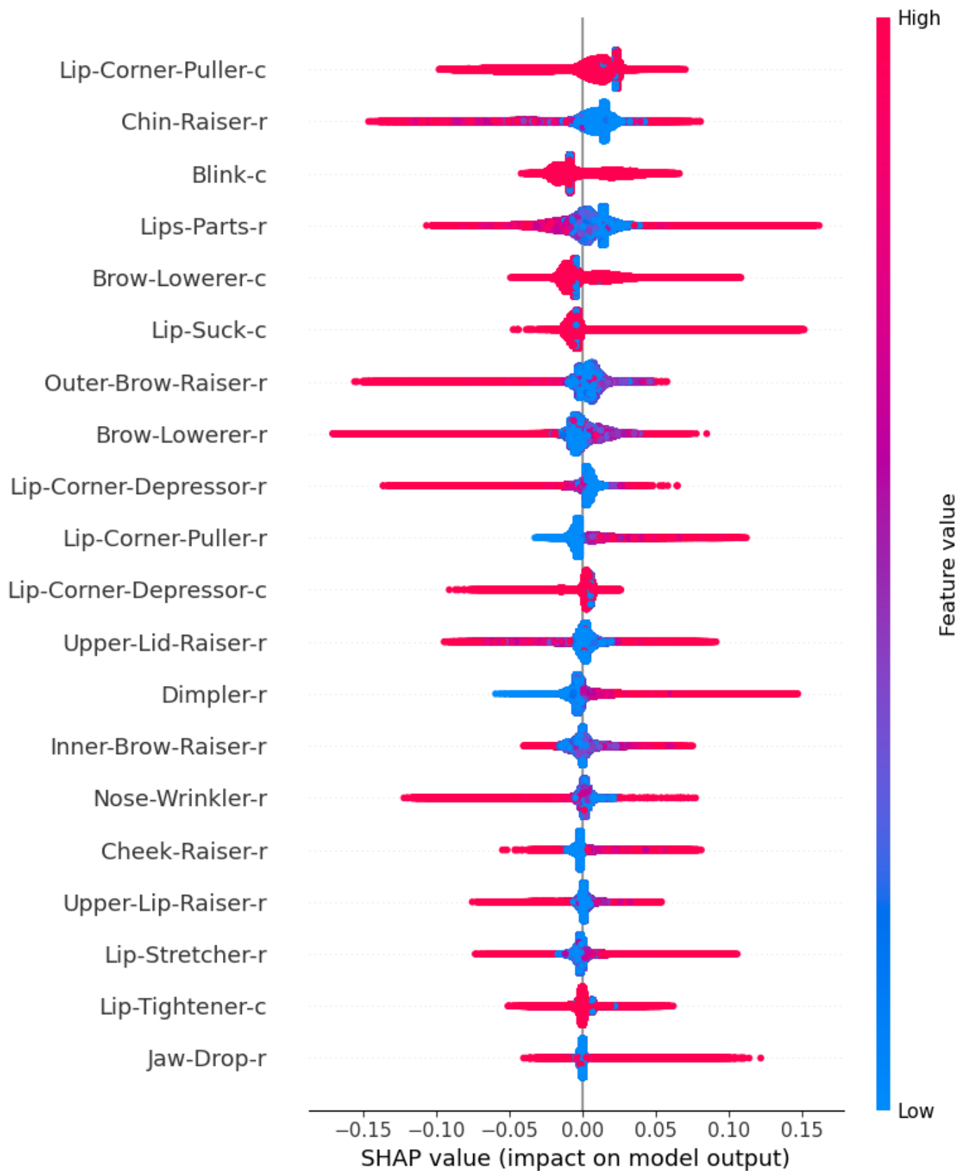
Fig. S35. Twenty most important features for AUs-Men – Iteration 5.
