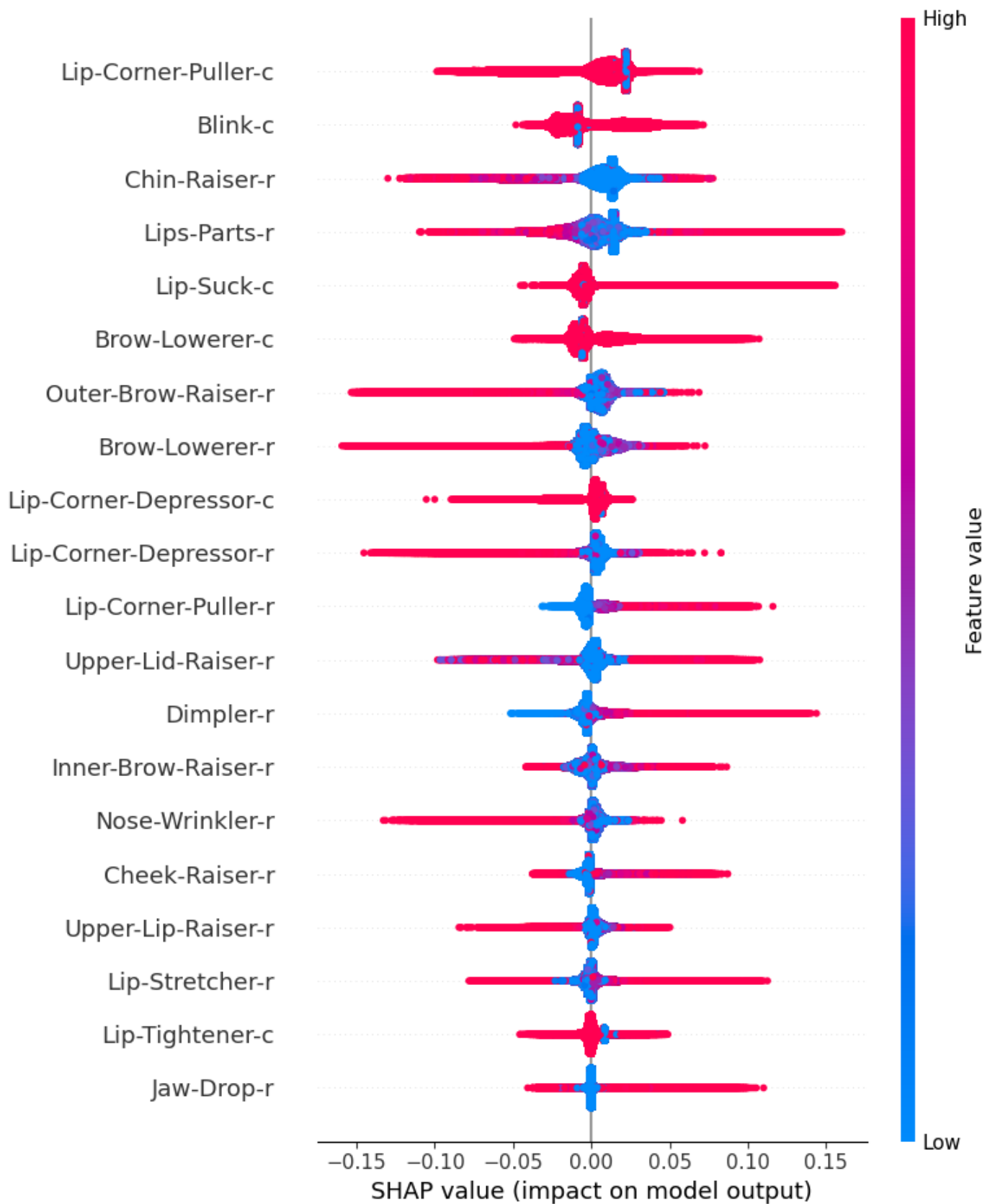
Fig. S32. Twenty most important features for AUs-Men – Iteration 2.
