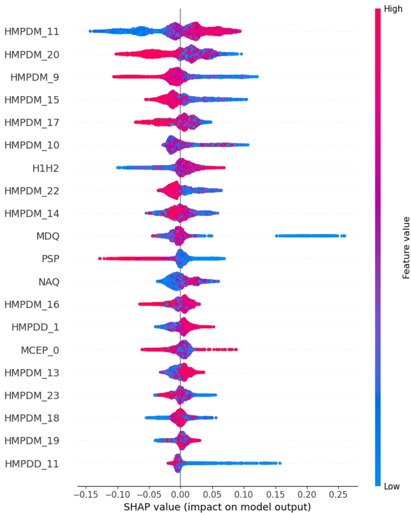
Fig. S14. Twenty most important features for Speech-Men – Iteration 4.
