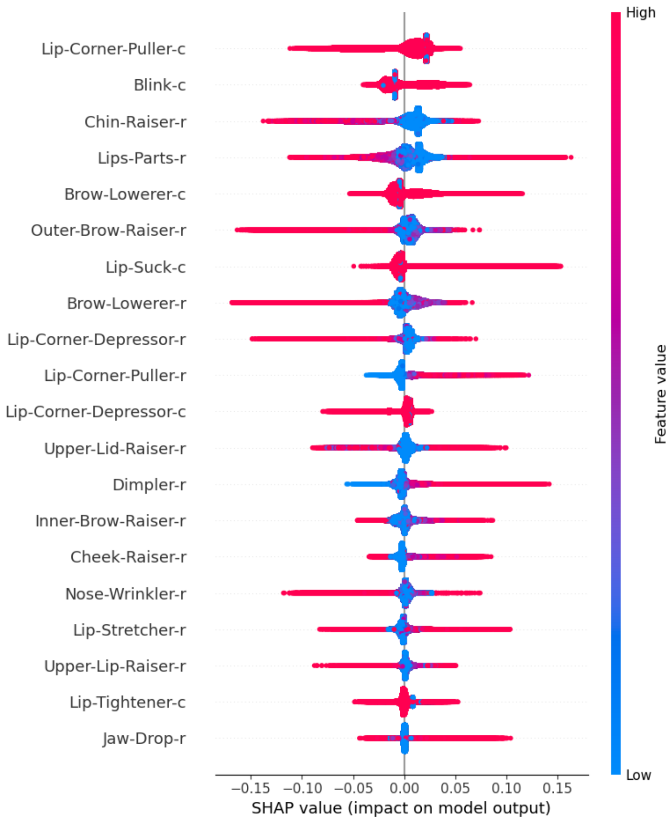
Fig. S38. Twenty most important features for AUs-Men – Iteration 8.
