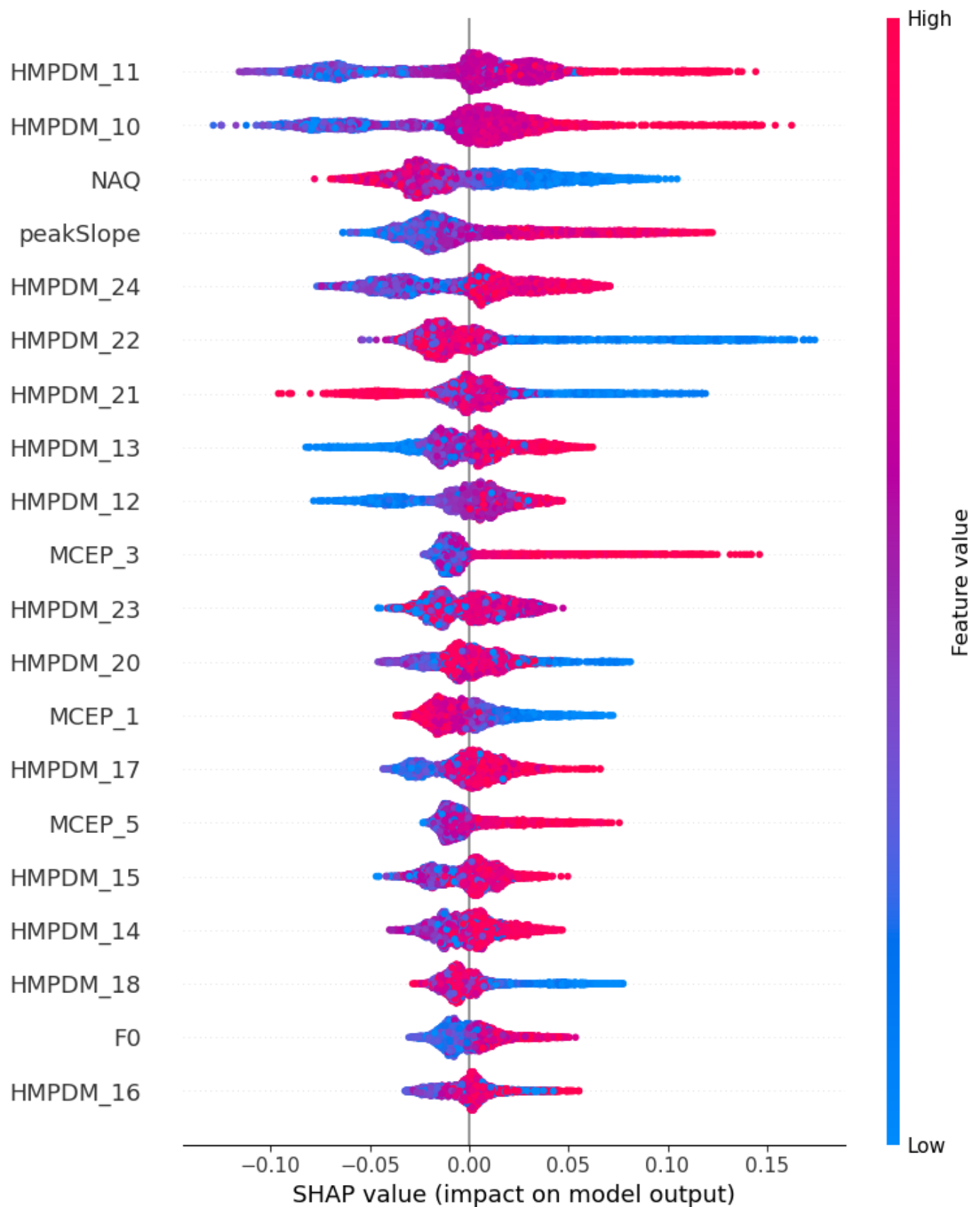
Fig. S1. Twenty most important features for Speech-Women – Iteration 1.
