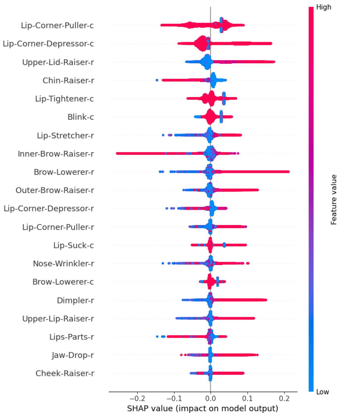
Fig. S24. Twenty most important features for AUs-Women – Iteration 4.
