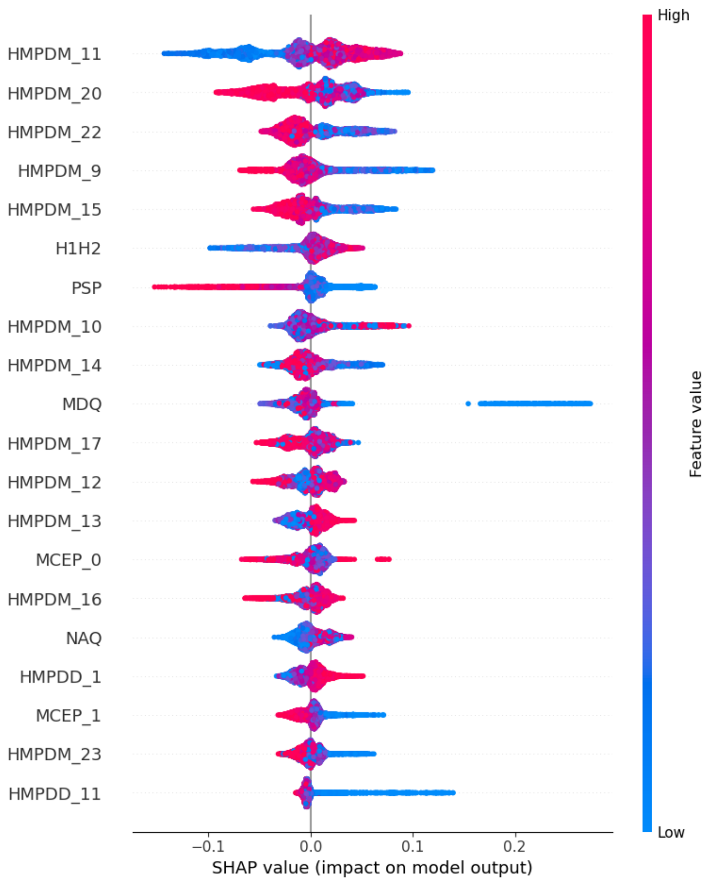
Fig. S18. Twenty most important features for Speech-Men – Iteration 8.
