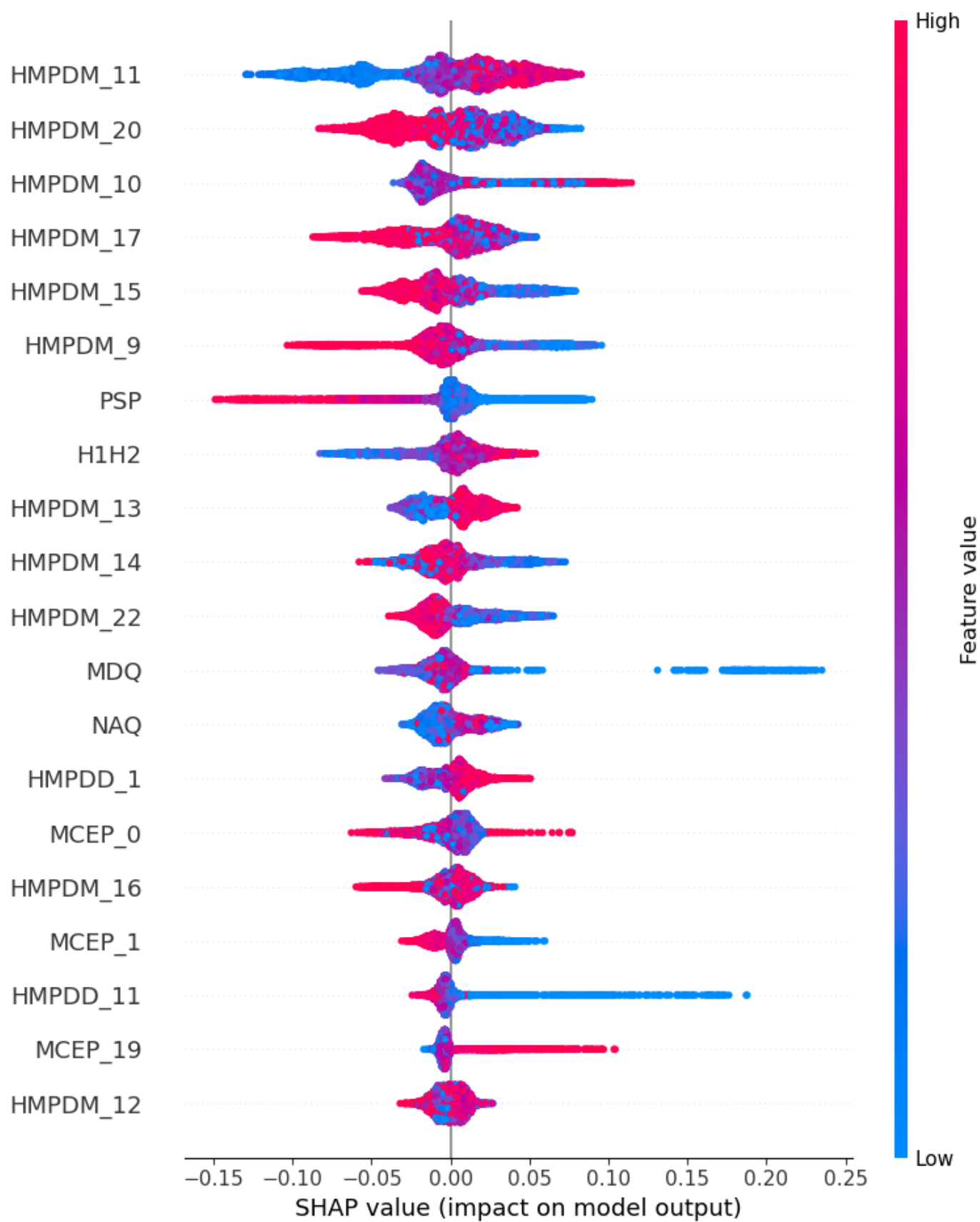
Fig. S15. Twenty most important features for Speech-Men – Iteration 5.
