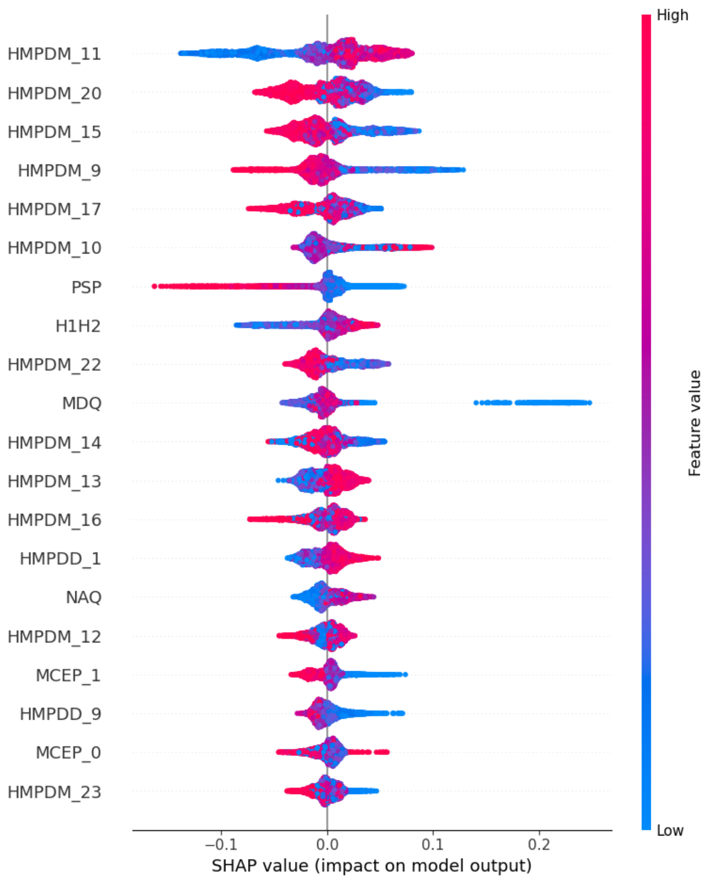
Fig. S13. Twenty most important features for Speech-Men – Iteration 3.
