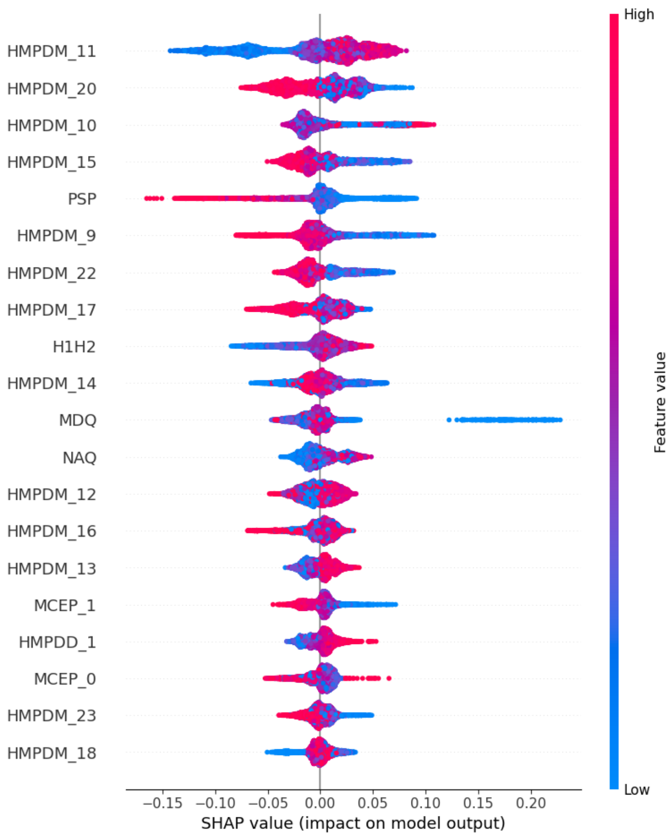
Fig. S20. Twenty most important features for Speech-Men – Iteration 10.
