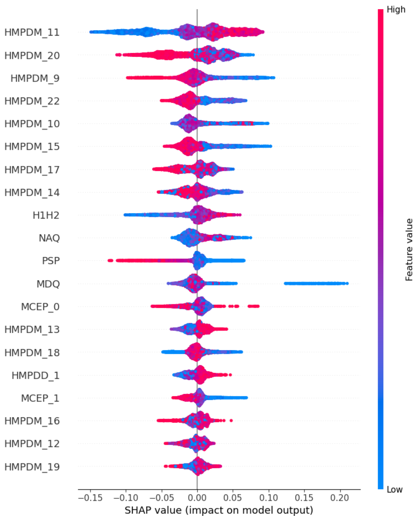
Fig. S17. Twenty most important features for Speech-Men – Iteration 7.
