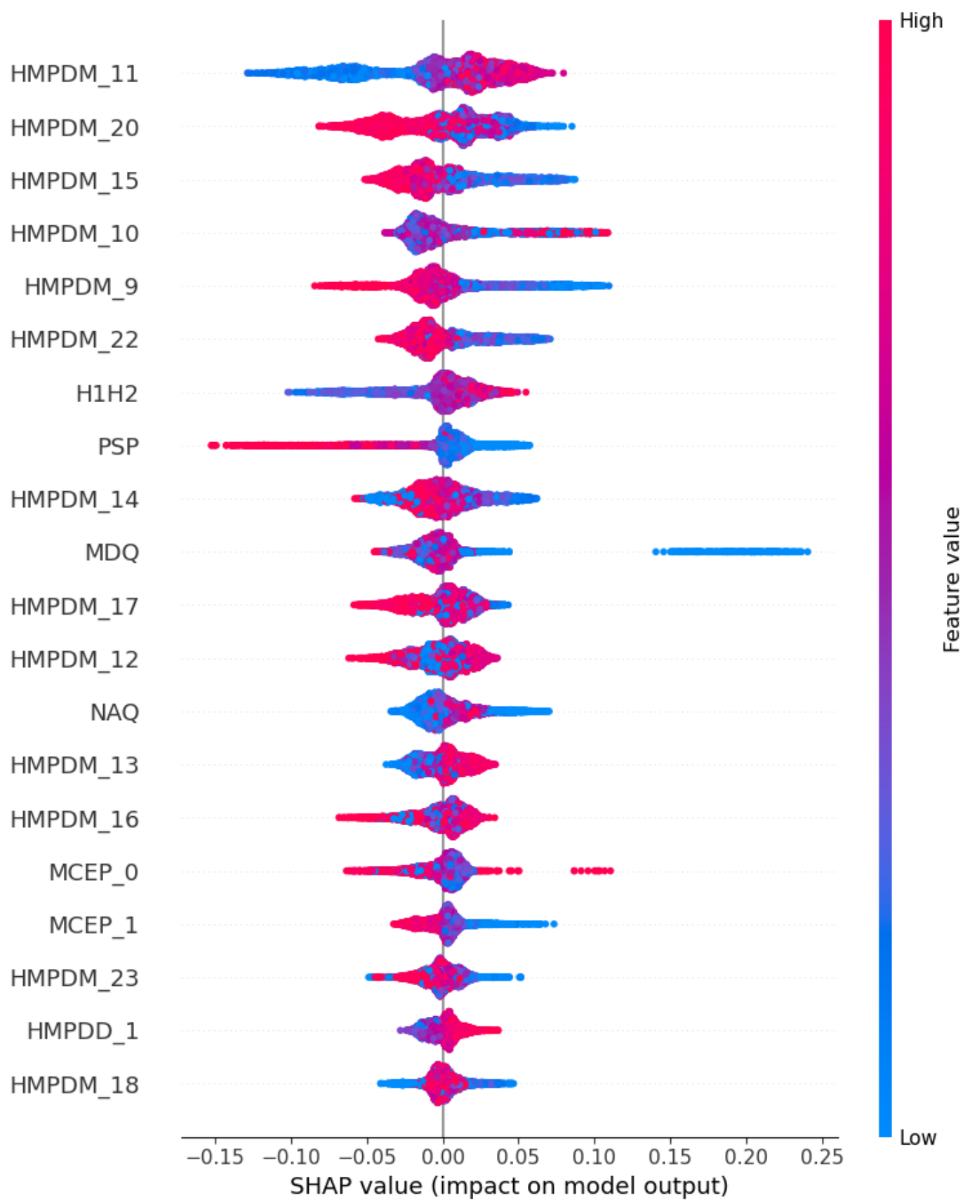
Fig. S16. Twenty most important features for Speech-Men – Iteration 6.
