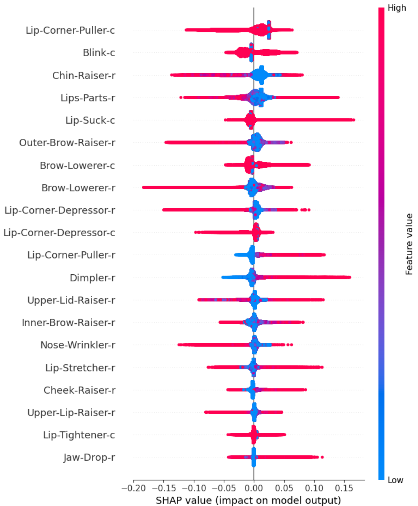
Fig. S39. Twenty most important features for AUs-Men – Iteration 9.
