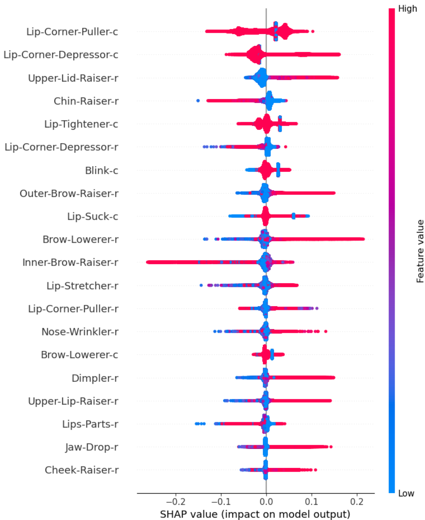
Fig. S21. Twenty most important features for AUs-Women – Iteration 1.
