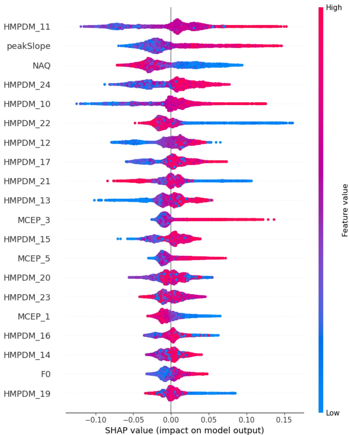
Fig. S4. Twenty most important features for Speech-Women – Iteration 4.
