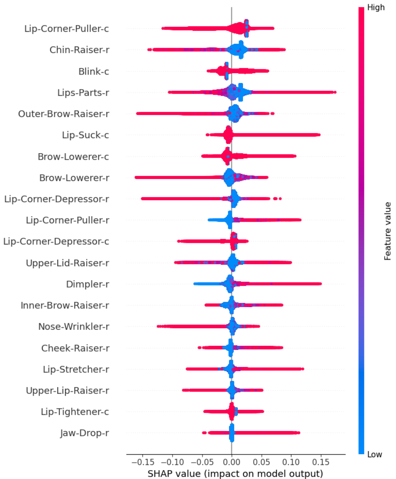
Fig. S33. Twenty most important features for AUs-Men – Iteration 3.
