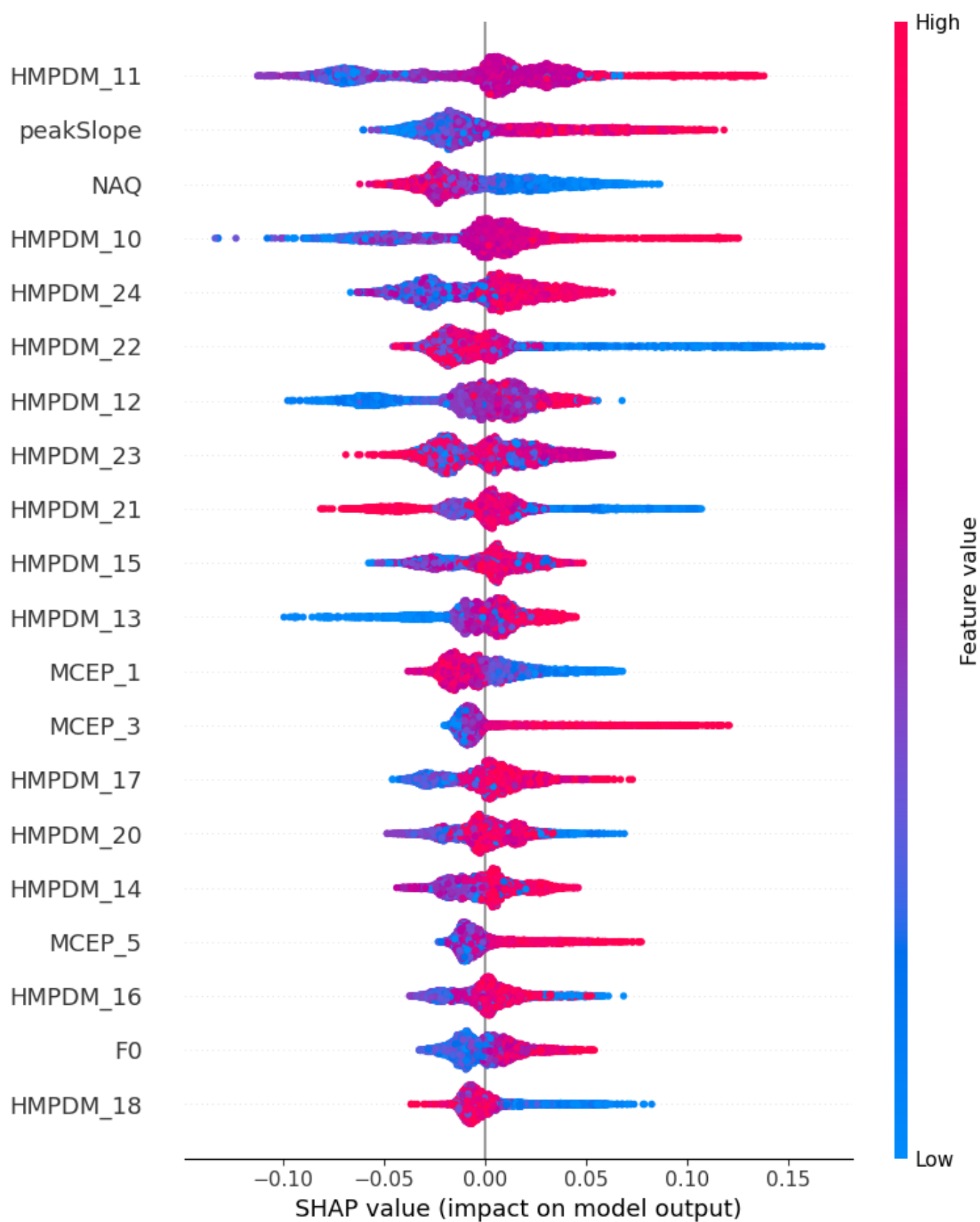
Fig. S3. Twenty most important features for Speech-Women – Iteration 3.
