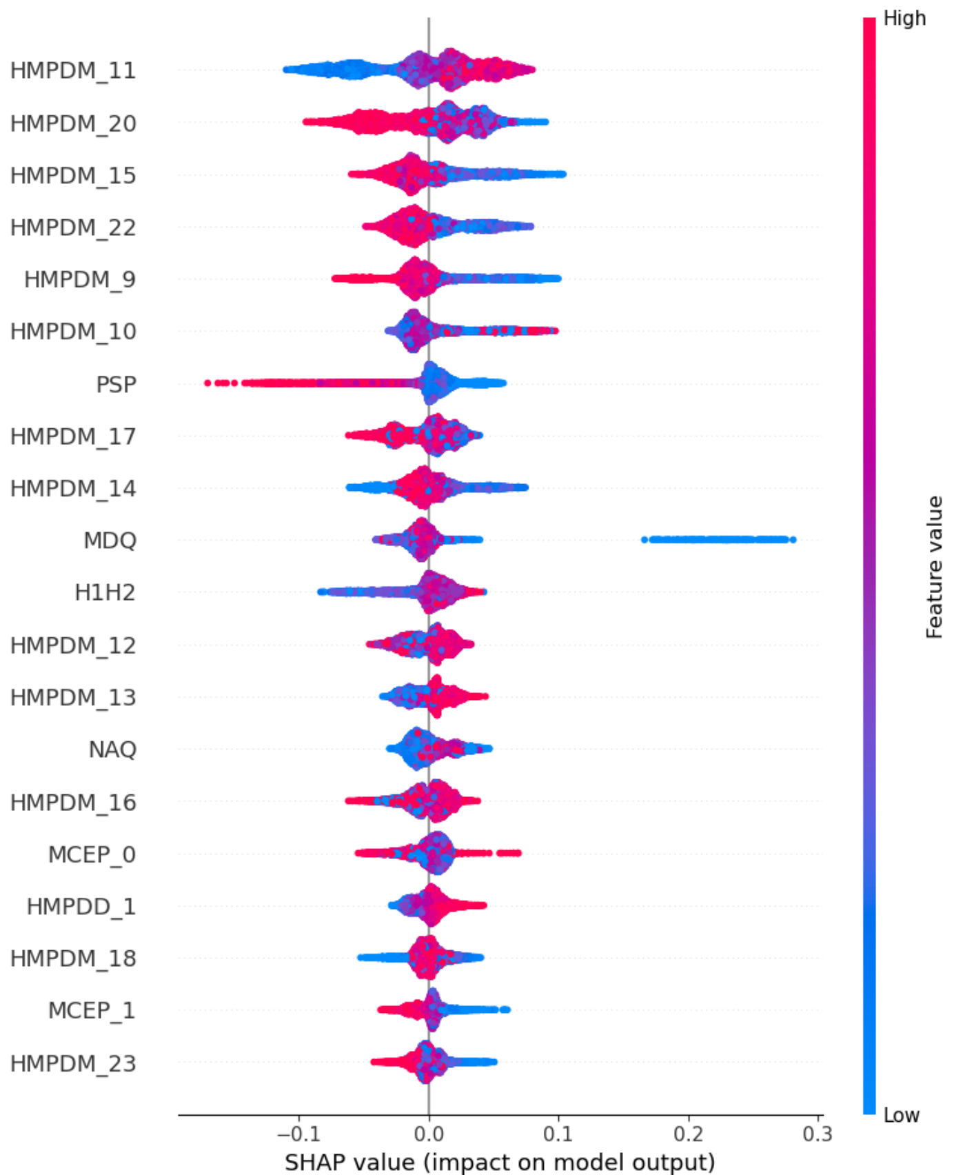
Fig. S11. Twenty most important features for Speech-Men – Iteration 1.
