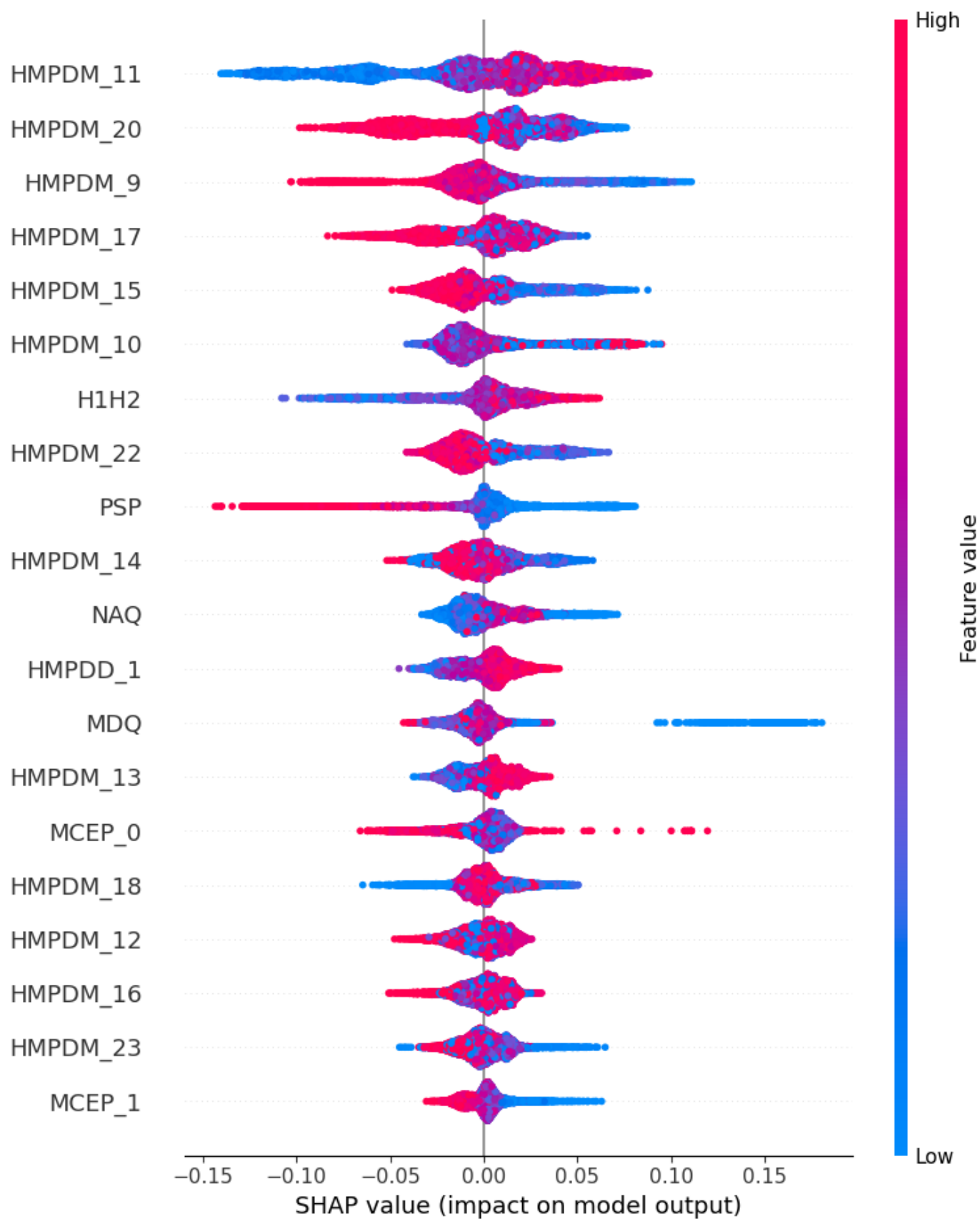
Fig. S12. Twenty most important features for Speech-Men – Iteration 2.
