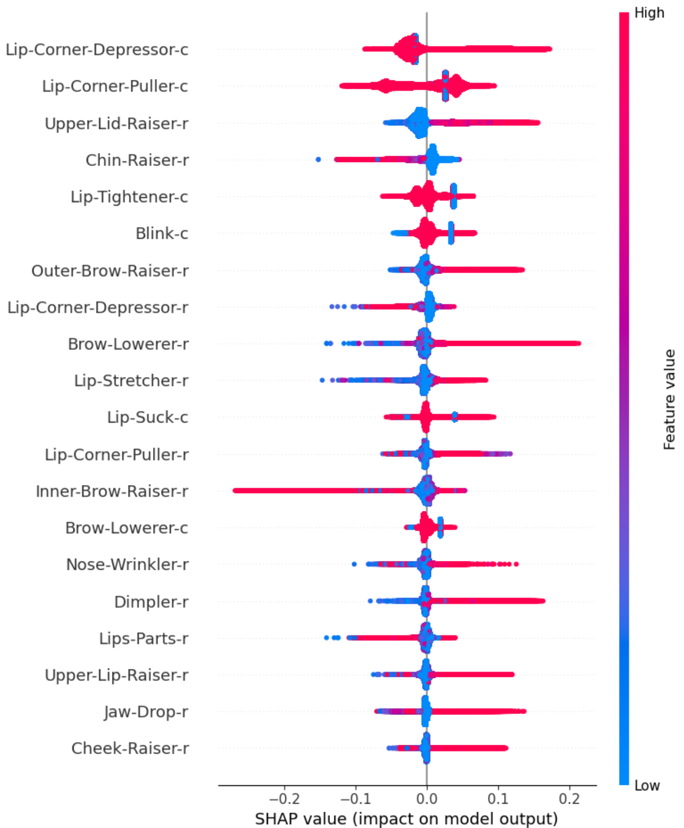
Fig. S30. Twenty most important features for AUs-Women – Iteration 10.
