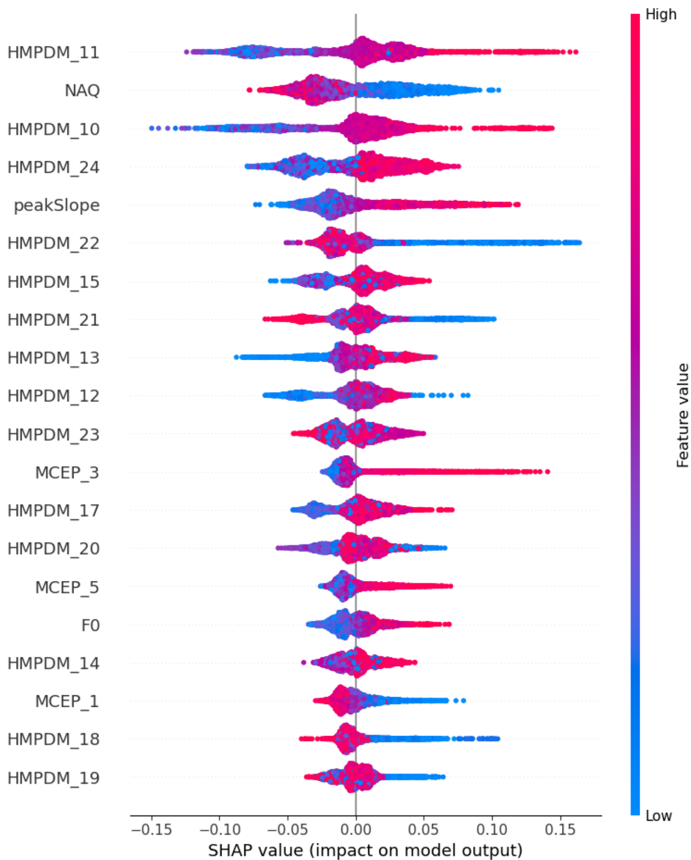
Fig. S2. Twenty most important features for Speech-Women – Iteration 2.
