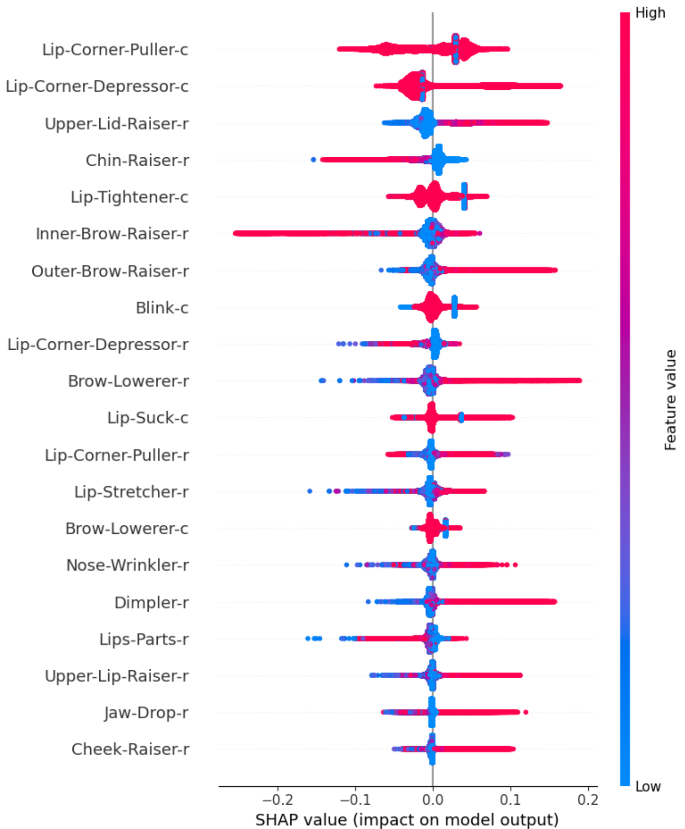
Fig. S26. Twenty most important features for AUs-Women – Iteration 6.
