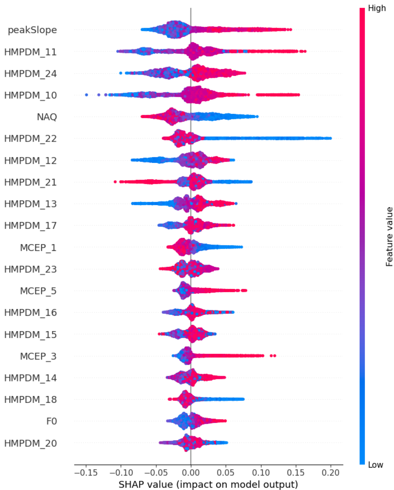
Fig. S5. Twenty most important features for Speech-Women – Iteration 5.
