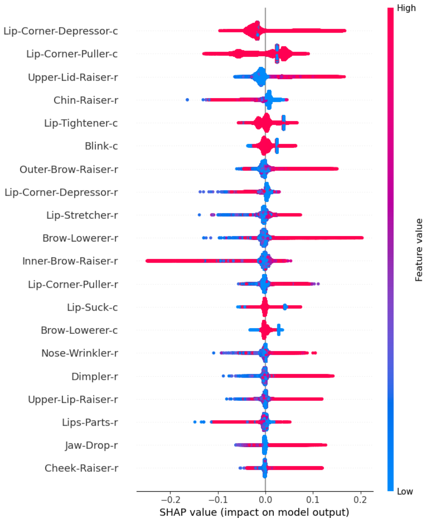
Fig. S22. Twenty most important features for AUs-Women – Iteration 2.
