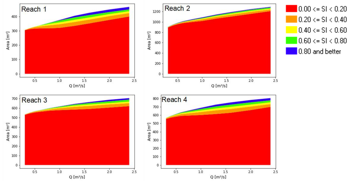
Figure S 1: Integrated habitat results SI areas chart for adult snow trout.
