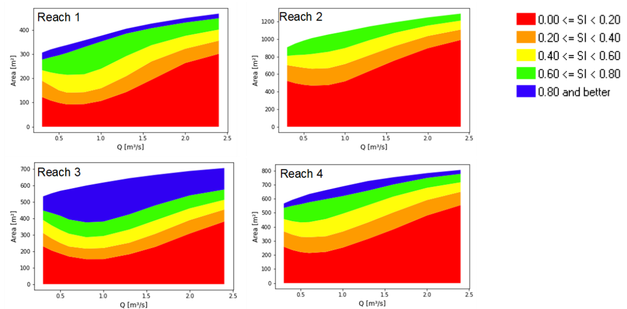
Figure S 2: Integrated habitat results SI areas chart for juvenile snow trout.
