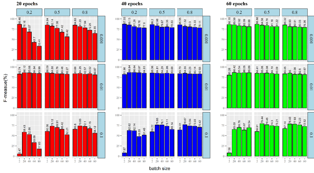
Fig. S1 Results for each configuration of the parameters of BiLSTM-CRF model in the hyper-parameter fine-tuning stage. The values used for the batch size were 2, 20, 40, 60 and 80; for the number of epochs were 20, 40 and 60, applying early stopping; for the dropout were 0.2, 0.5 and 0.8; and for the learning rate were 0.1, 0.01 and 0.001, with the Adam algorithm. BiLSTM-CRF bidirectional long short-term memory conditional random field
