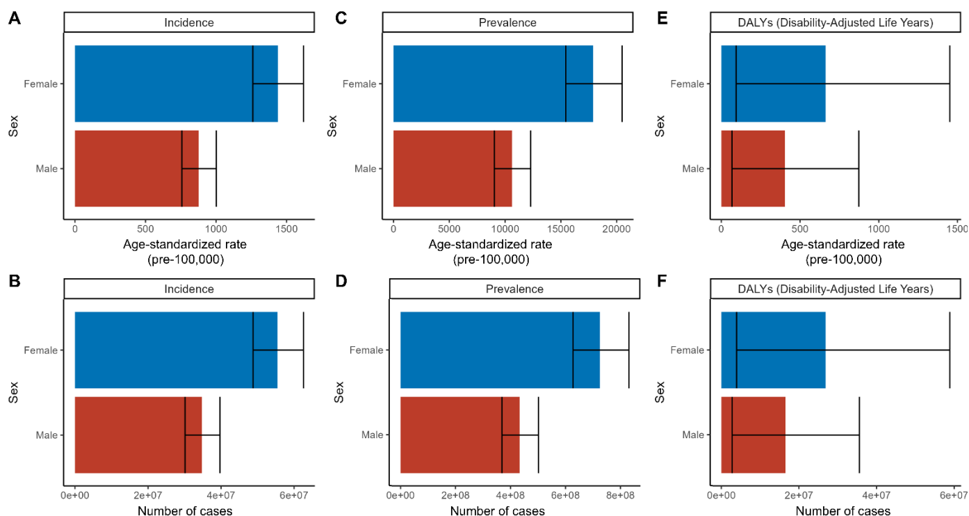
Supplementary Fig. S2 Global burden of migraine by sex, 2021. ASIR (A) and incidence cases (B) , ASPR (C) and prevalence cases (D) , ASDR (E) and DALYs cases (F) for migraine in 2021.
