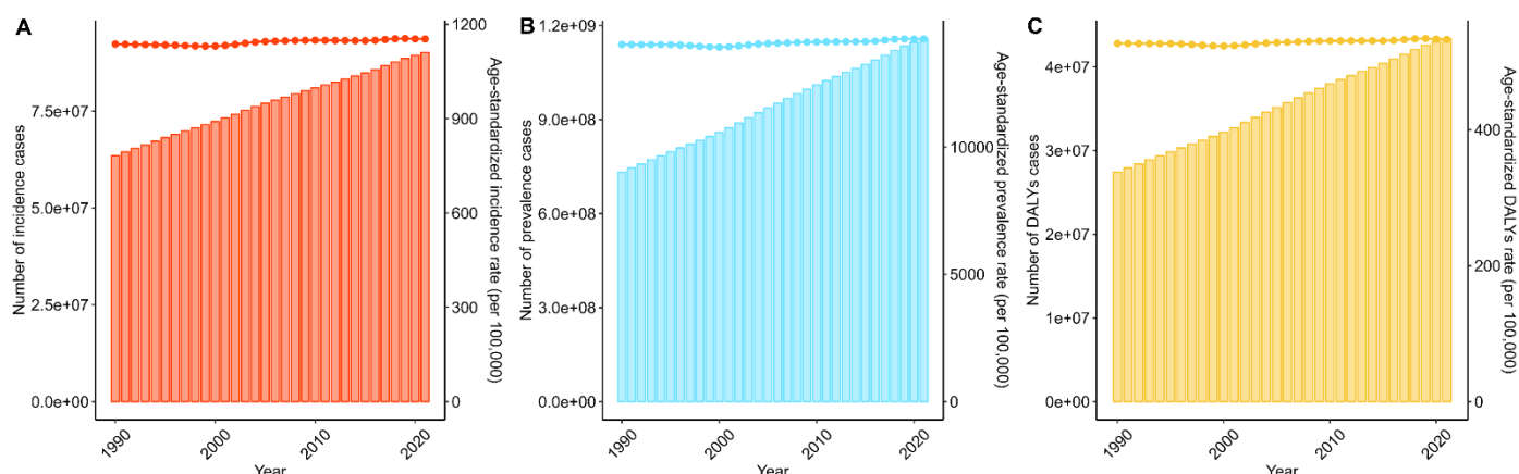
Supplementary Fig. S1 Trend in global burden of migraine from 1990 to 2021. (A) Trend in the incidence cases and ASIR; (B) Trend in the prevalence cases and ASPR; (C) Trend in the DALYs cases and ASDR.
